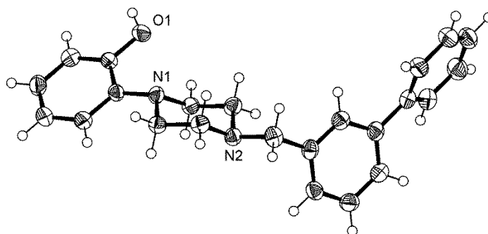
Figure 1. X-Ray crystal structure of 3
