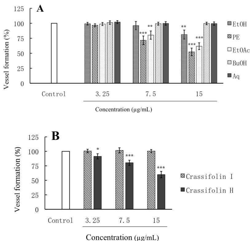
Figure 3. Anti-angiogenic activities of the EtOH extracted and its four sub-fractions (PE, EtOAc, BuOH and Aq fractions) of C. crassifolius ( A ) and the isolated compounds (crassifolin I and crassifolin H) from EtOAc fractions ( B ). Effects were assessed by measuring the vessel formation of samples as compared to the control (0.2% DMSO was used as carrier control) using the quantitative EAP assay. Data are expressed as means \pm standard deviation ( n = 10 ). Mean values of sample show significant different from the control group was denoted with * ( p < 0.05 ), ** ( p < 0.01 ), and *** ( p < 0.001 ) in one-way ANOVA followed by Dunnett's test.
