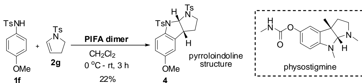
Scheme 5. One-step formation of pyrroloindoline 4 from anilide utilizing cyclic enamide 2g
