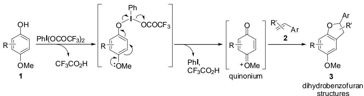
Scheme 1. General mechanism of oxidative phenolic coupling with styrenes leading to dihydrobenzofurans using hypervalent iodine reagent
