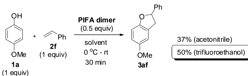
Scheme 3. Solvent effect
