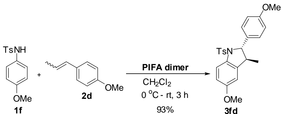
Scheme 4. Construction of indoline structure from anilide 1f
