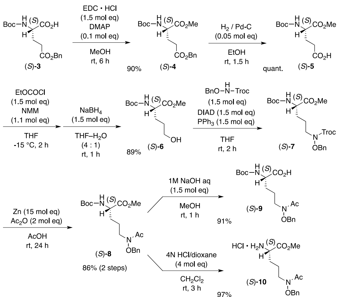
Scheme 1. Synthesis of amino acid building blocks ( S )- 9 and ( S )- 10
