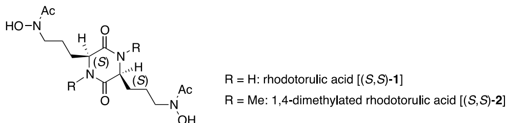
Figure 1. Rhodotorulic acid [( S,S )- 1 ] and its 1,4-dimethylated derivative [( S,S )- 2 ]
