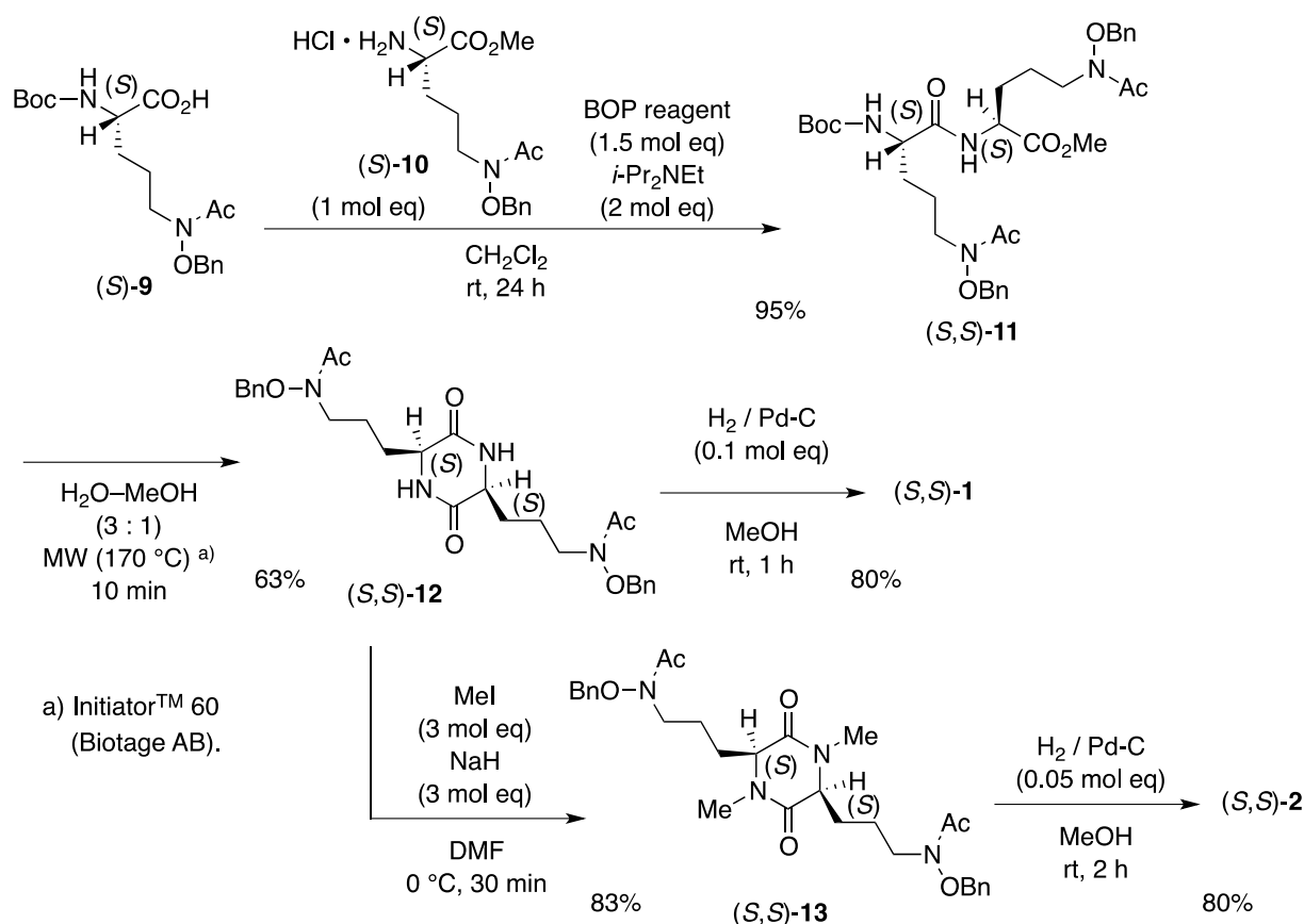
Scheme 2. Synthesis of rhodotorulic acid [(S,S)-1] and its 1,4-dimethylated derivative [(S,S)-2]
