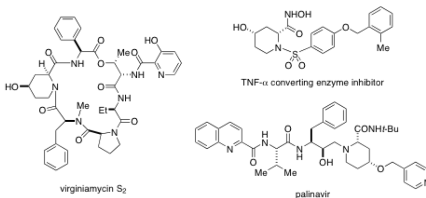
Figure 1. Selected biologically active compounds having 4-hydroxypipercolinic acid fragment
