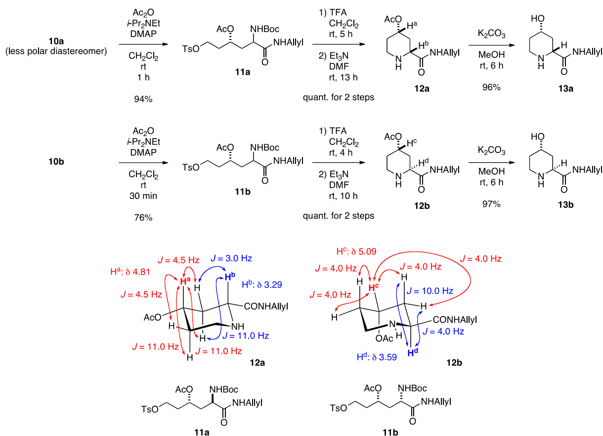
Scheme 2. Transformation into pipercolinic acid derivatives
