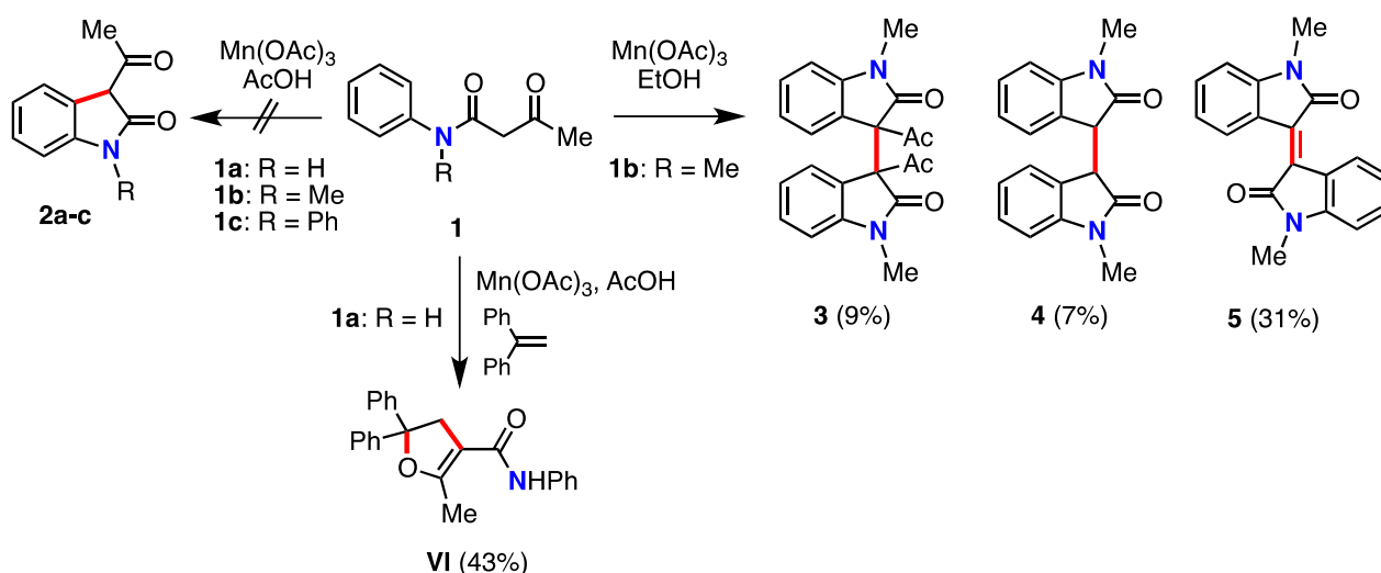
Scheme 2. Reaction of 3-Oxo- N -phenylbutanamides 1a–c with Mn(OAc) 3
