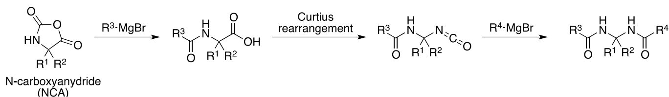
Scheme 2. Synthesis of unsymmetrical, gem -disubstituted bisamides via addition of Grignard reagents to isocyanates
