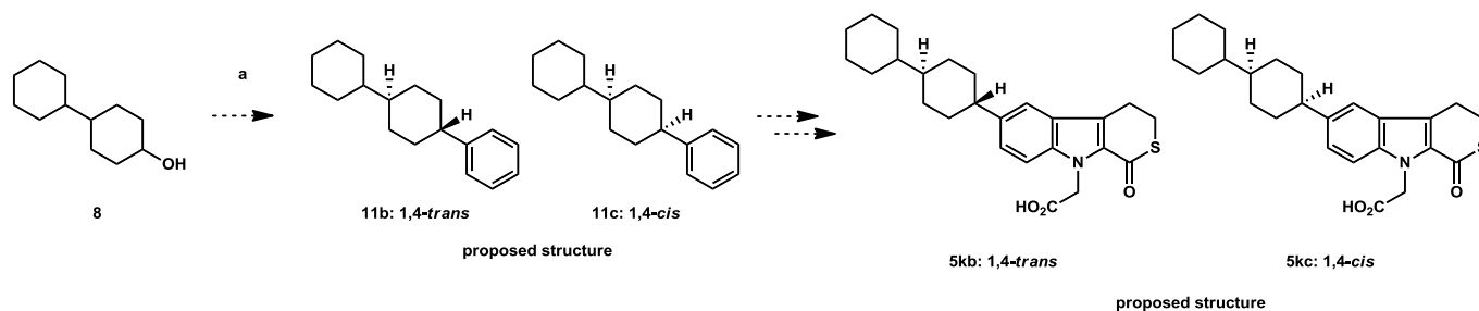
Scheme 3. Reagents and conditions: (a) \text{AlCl}_3 , PhH
