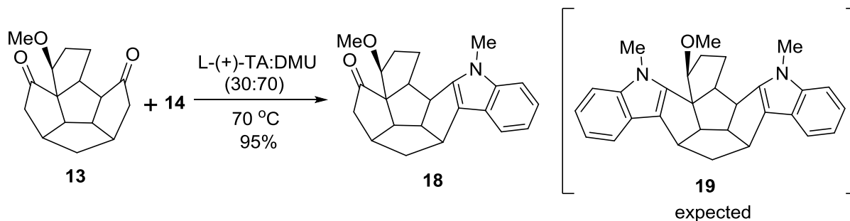
Scheme 4. Synthesis of aza-polyquinane 18
