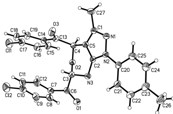
Figure 1. X-Ray structure of 3a 10
