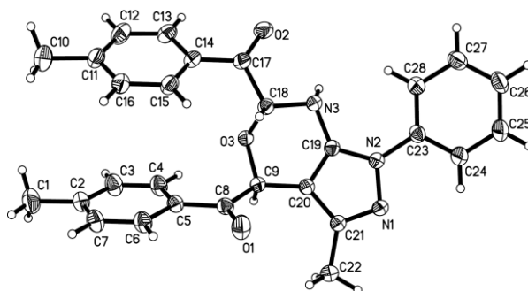
Figure 2. X-Ray structure of 3b 11
