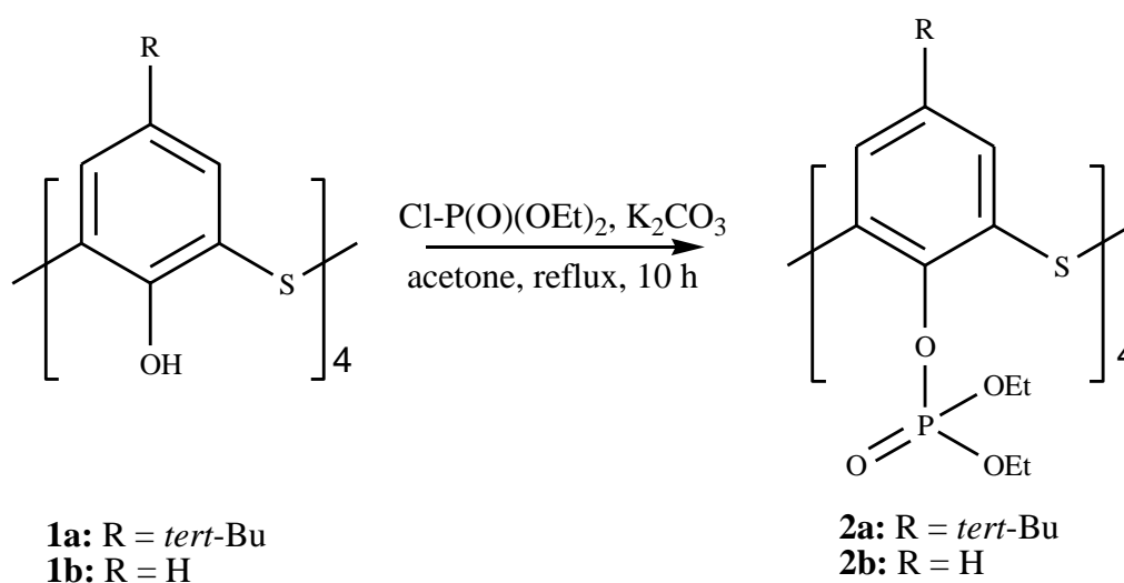
Scheme 1. Synthesis of TC4A-Phosphates (2a & 2b)
