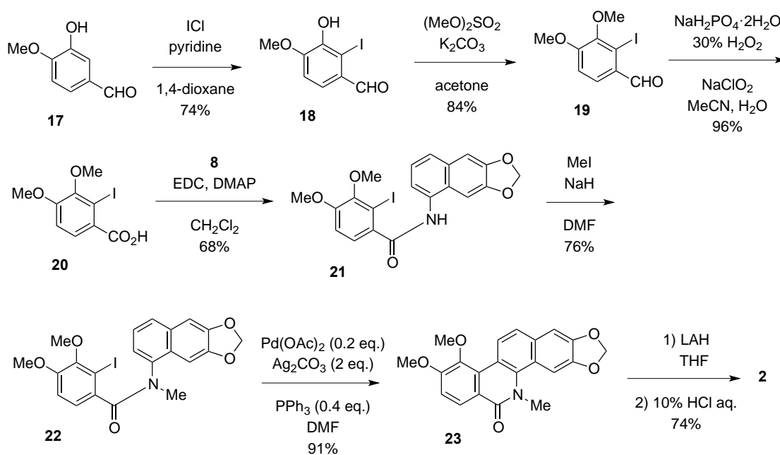
Scheme 3. Synthesis of 2 via Pd-mediated Aryl-Aryl Coupling Reaction
