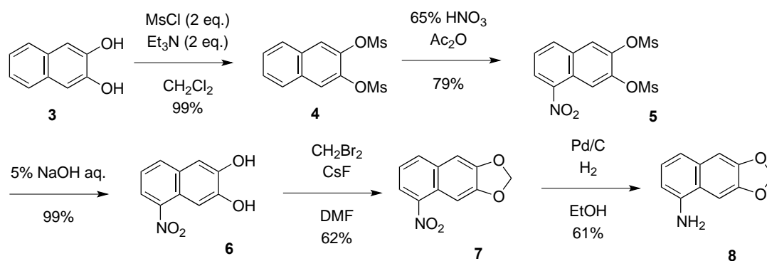
Scheme 1. Preparation of 1-Naphtylamine
