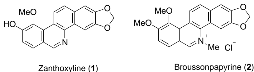
Figure. Originally Reported Structures of Zanthoxyline ( 1 ) and Broussonpapyrine ( 2 )
