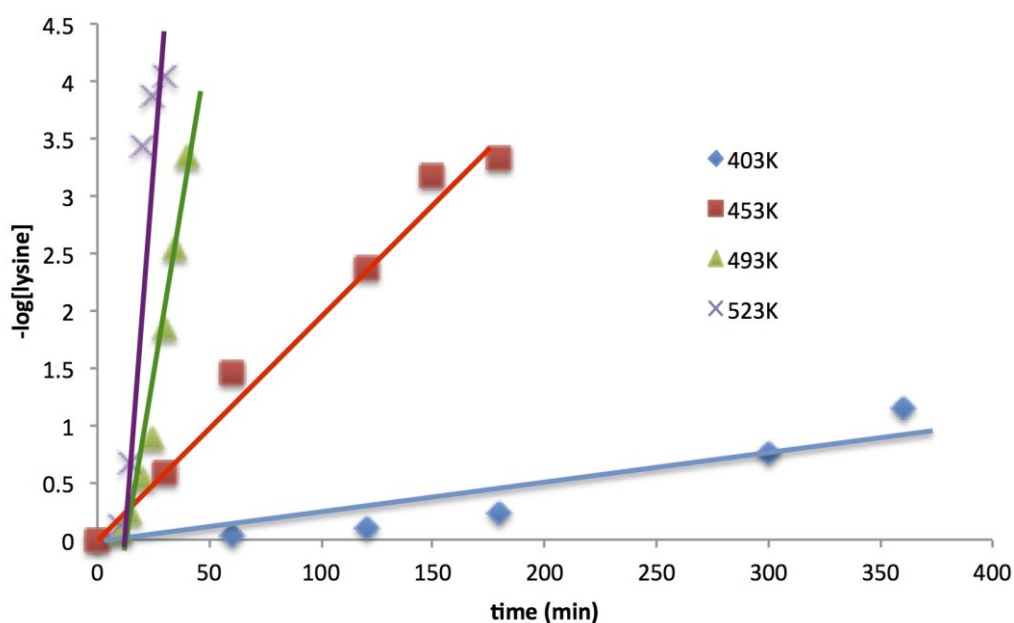
Figure 2. -\log[1] -reaction time plots
