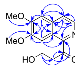
Figure 2. Key HMBC ( \curvearrowright ) correlations of 1
