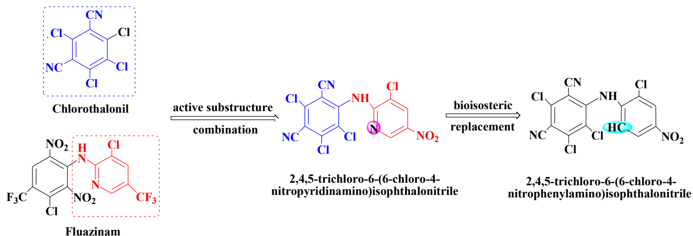
Scheme 2. Design of novel aniline derivatives of Chlorothalonil
