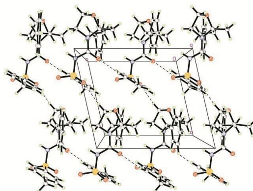
Figure 2. Packing diagram of finacompound 4d in a unit cell
