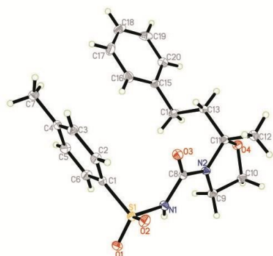
Figure 1. Molecular structure of product 4d
