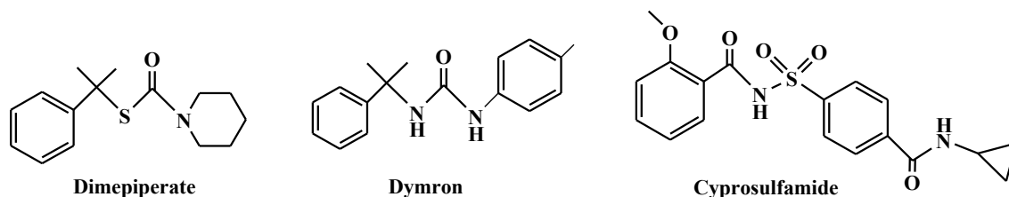
Scheme 1. Safeners for sulfonylurea herbicides
