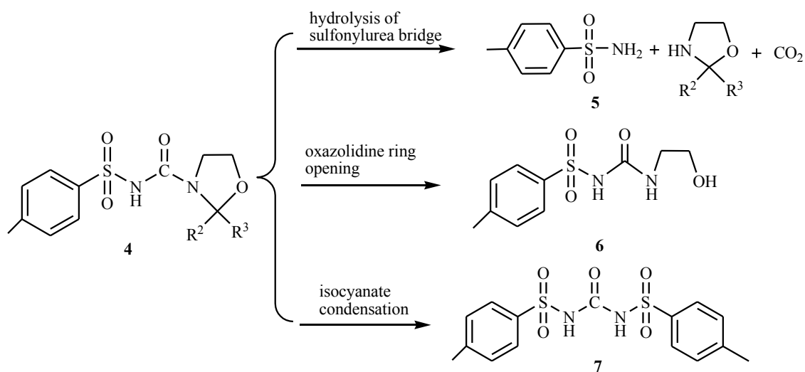
Scheme 5. The schematic diagram of the cleavage products
