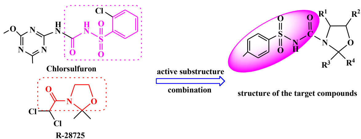
Scheme 3. Design of the target compound
