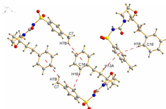
Figure 3. C-H... \pi interactions of the compound 4d
