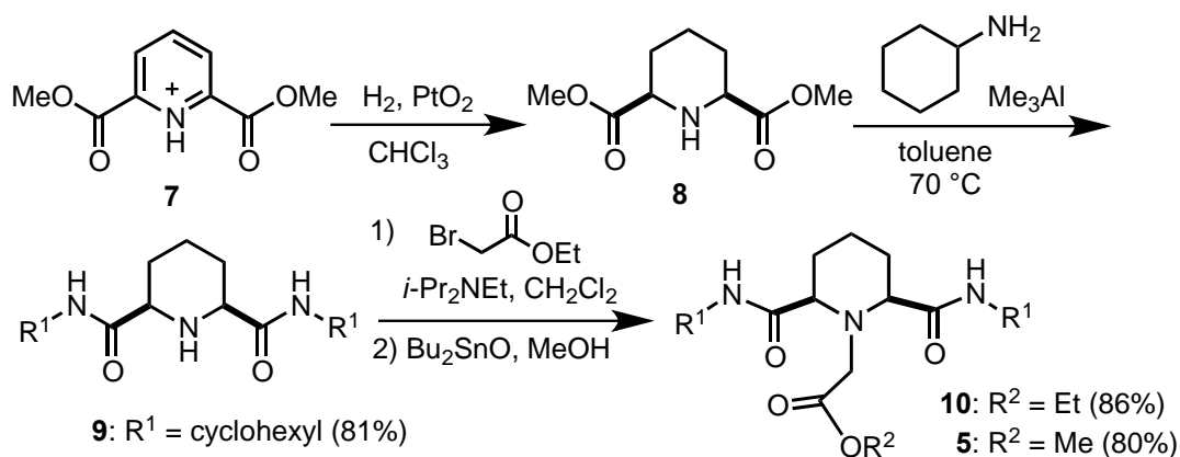
Scheme 2. Synthesis of cis -2,6-piperidinedicarboxamide 5
