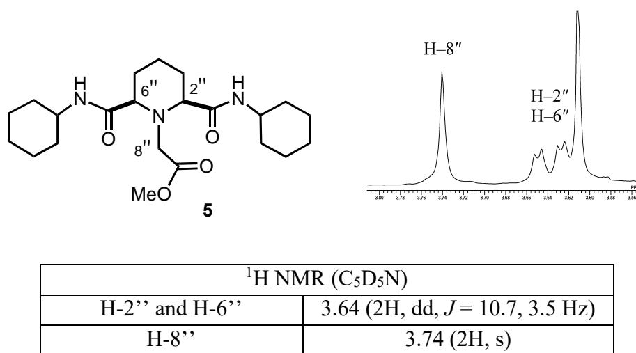
Figure 3. ^1\text{H} NMR spectra and data for the cis -2,6-piperidinedicarboxamide 5
