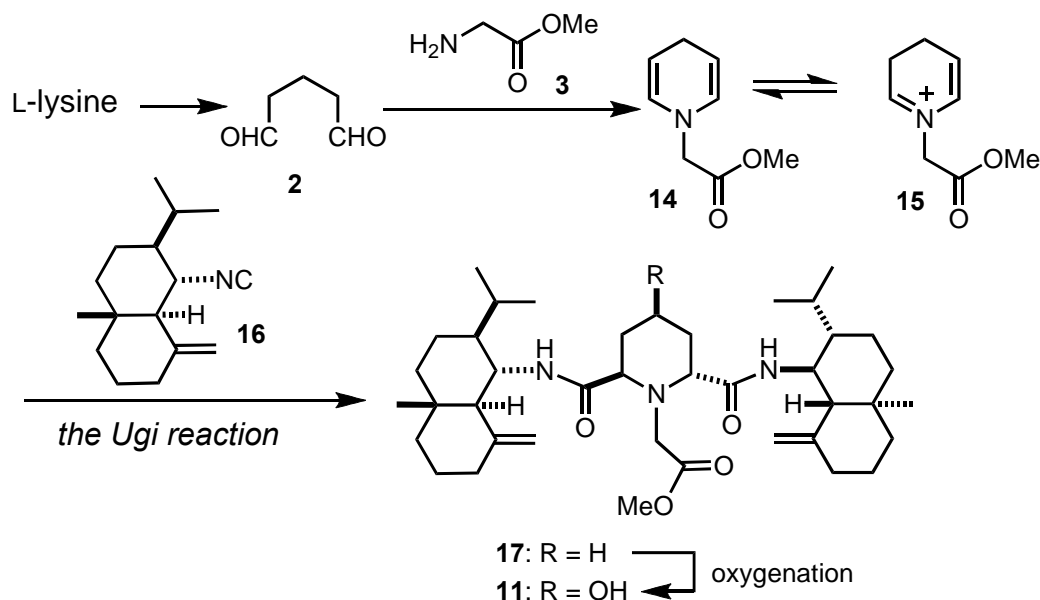
Scheme 4. Plausible pathway for the biosynthesis of halichonadin P
