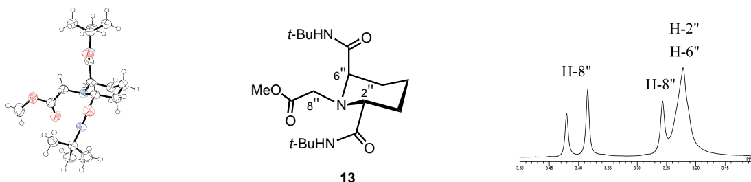
Figure 5. ORTEP plot of the X-ray data and selected 1 H NMR (CDCl 3 ) of 13
