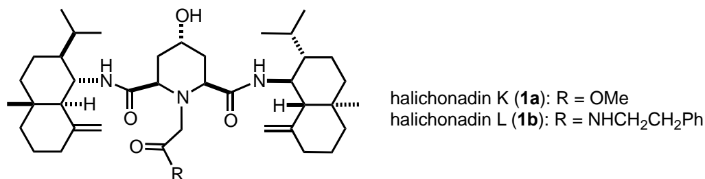
Figure 1. Structures of halichonadins K and L
