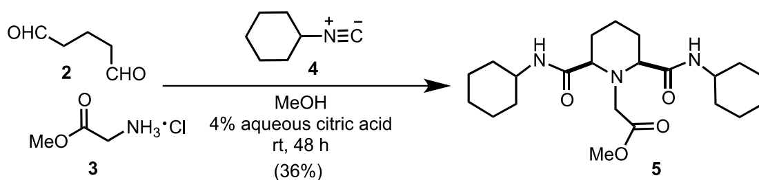
Scheme 1. One-pot three-component reaction reported by Poupon
