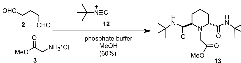
Scheme 3. One-pot synthesis of the central core of halichonadin P
