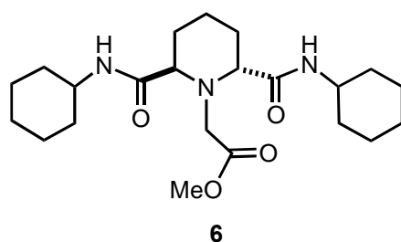
Figure 2. A newly proposed structure of the Poupon's product
