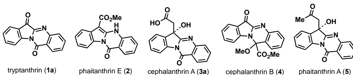
Figure 1. Indoloquinazoline alkaloids
