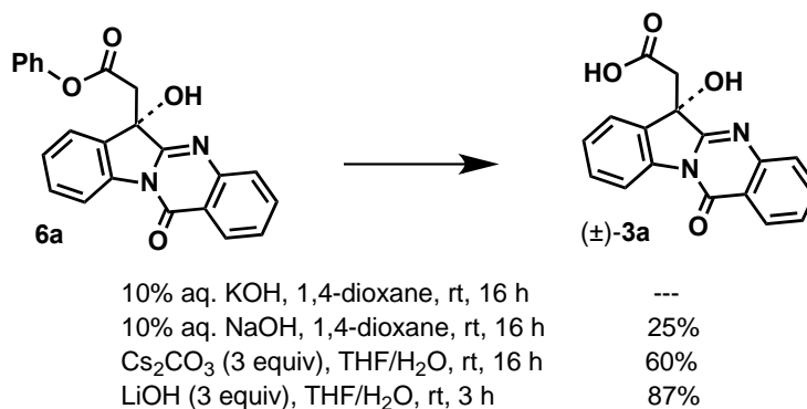
Scheme 3
