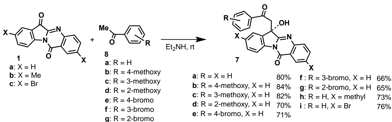
Scheme 2
