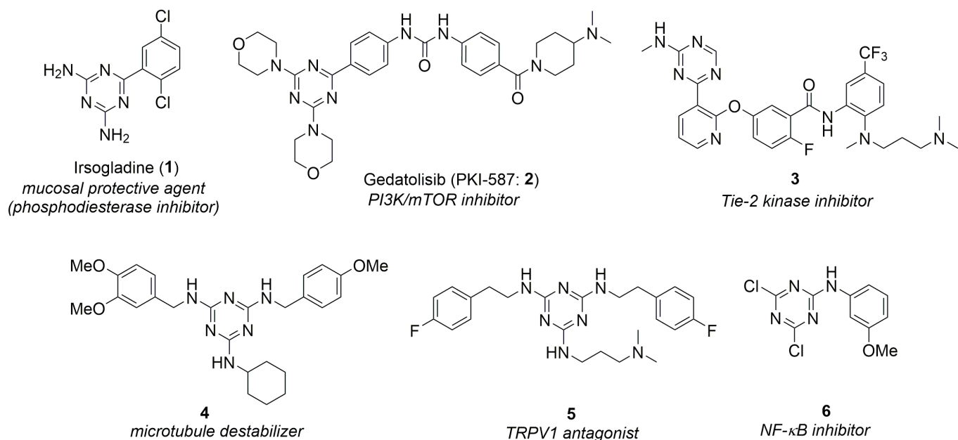
Figure 1. Examples of biologically active compounds bearing a 1,3,5-triazine moiety
