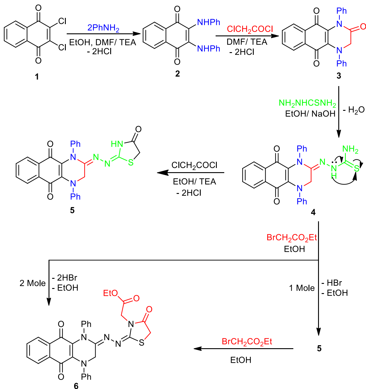
Scheme 1. Synthesis of thiazolidinone derivaives 5 and 6
