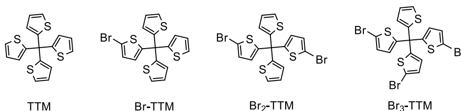
Figure 1. Tetra-2-thienylmethane (TTM) and its partially \alpha -brominated derivatives: Br-TTM, Br 2 -TTM, and Br 3 -TTM
