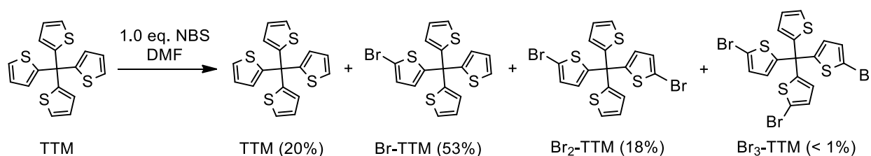
Scheme 1. Bromination of TTM with 1.0 equivalent NBS in DMF
