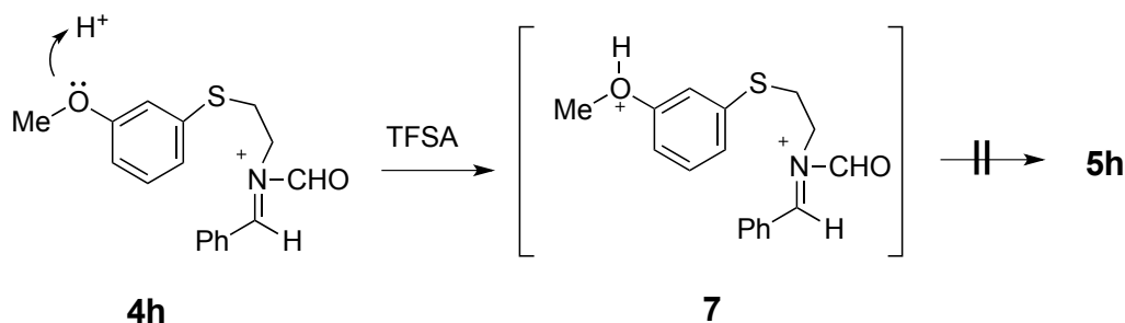
Scheme 2. Cyclization reaction of N -formyliminium ion ( 4h ) under mixed acid catalyzed (TFA-TFSA-Ac 2 O) reaction condition
