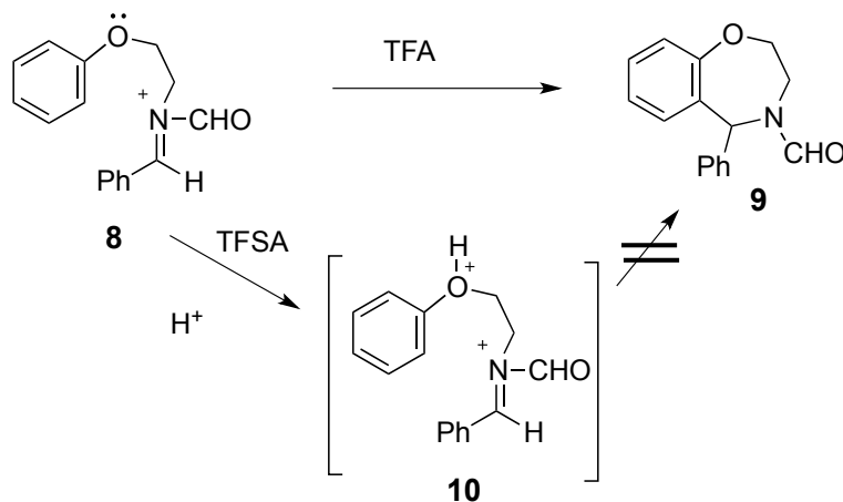
Scheme 3. Cyclization reaction of N -formyliminium ion ( 8 ) under acidic reaction condition
