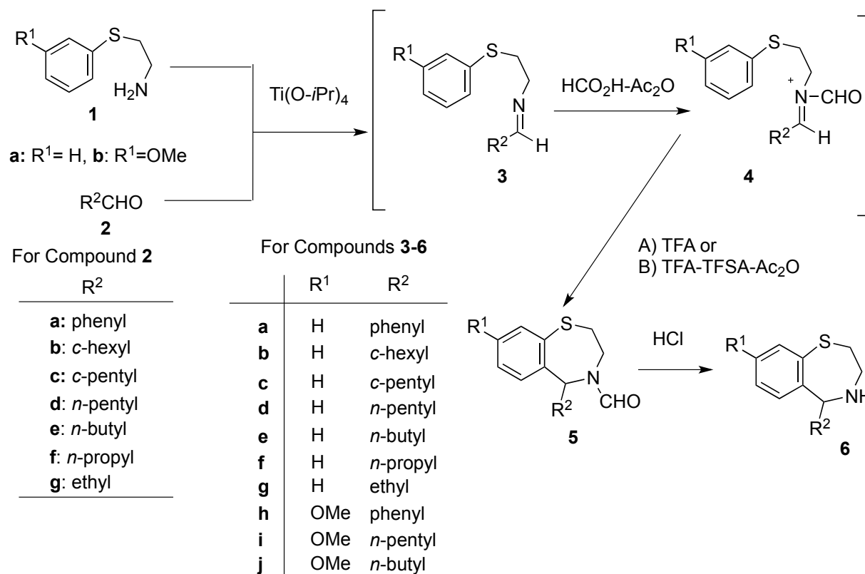
Scheme 1. Synthesis of 5-substituted-2,3,4,5-tetrahydrobenzo[ f ][1,4]thiazepines
