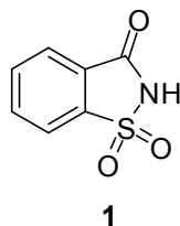
Figure 1. Structure of saccharin 1
