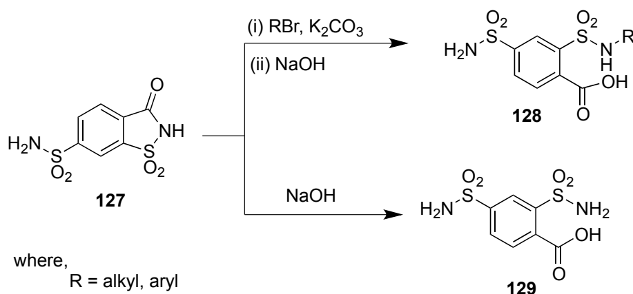
Scheme 31. Synthesis of bissulfamoylbenzoic acids 128 and 129 from 6-sulfamoylsaccharin 127
