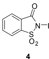
Figure 3. Structure of N -iodosaccharin 4
