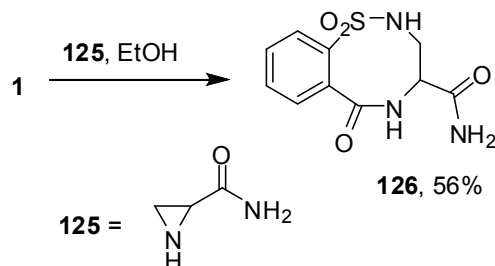
Scheme 30. Synthesis of the 8-membered heterocyclic compound 126 from saccharin 1 and leakadine 125
