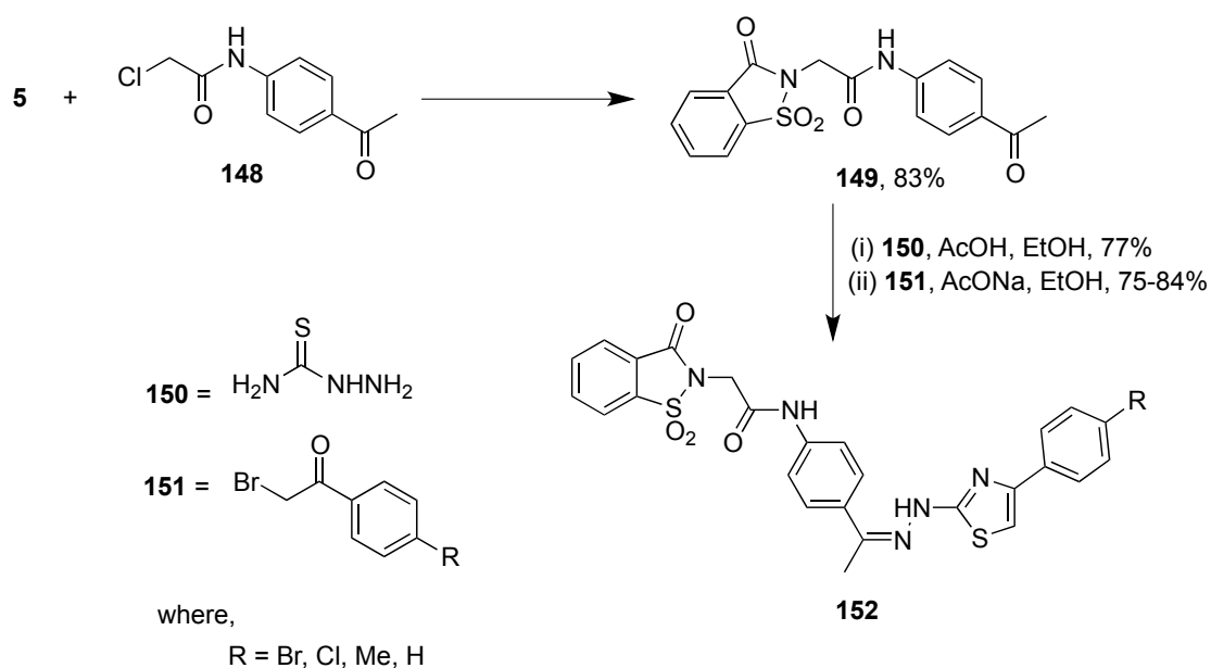
Scheme 36. Synthesis of a new series of benzisothiazolone 152 from sodium saccharin 5
