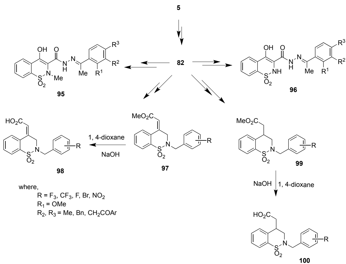
Scheme 23. Synthesis of the benzothiazinecarbohydrazide derivatives, 95 and 96 , and the benzothiazine-carboxylate derivatives ( 97-100 )
