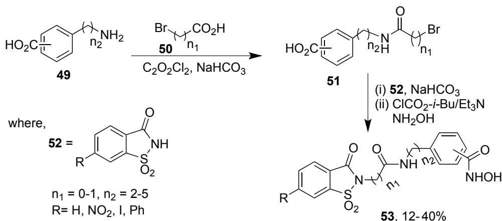
Scheme 13. Synthesis of N -hydroxybenzamide 53 from saccharin 52
