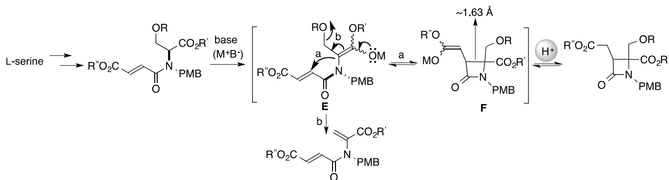
Scheme 4
