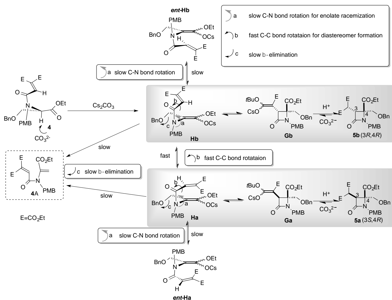
Scheme 7
