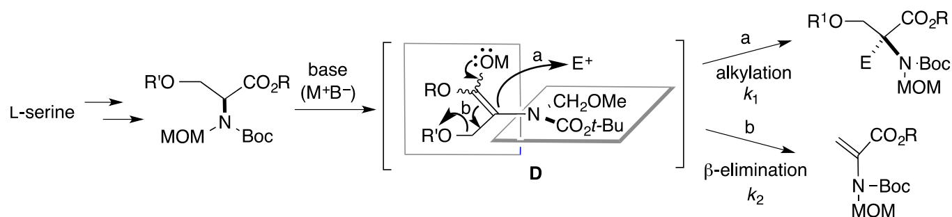
Scheme 3
