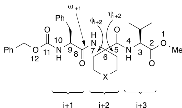
Figure 3. Numbering of the atoms (arbitrary) and torsion angles of the peptide backbone of 10a and 10c
