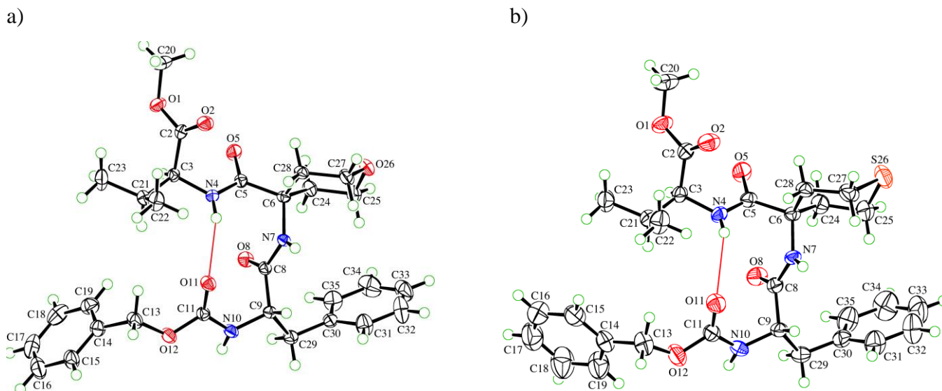
Figure 2. ORTEP plots 16 of the molecular structures of the tripeptides a) Z-Phe-Thp-Val-OMe ( 10a ) and b) Z-Phe-Tht-Val-OMe ( 10c ). Displacement ellipsoids are drawn at the 50% probability level.
