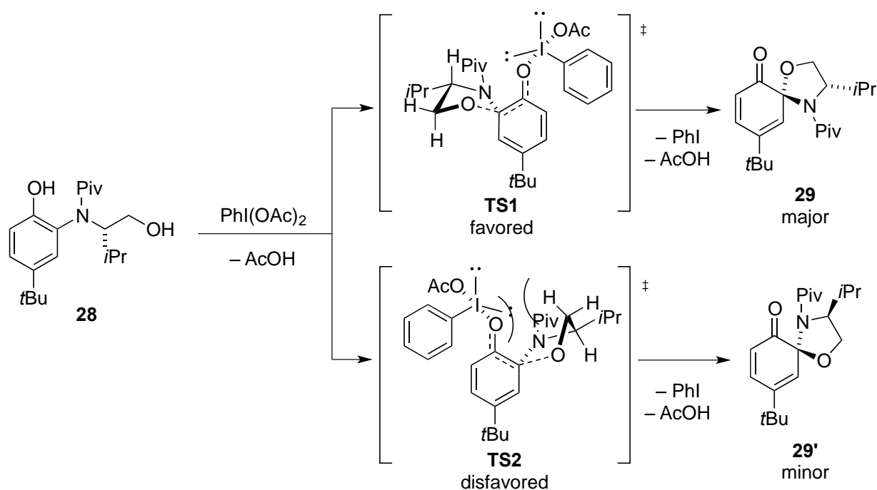
Scheme 10. Proposed rationale for the stereoselective formation of 29
