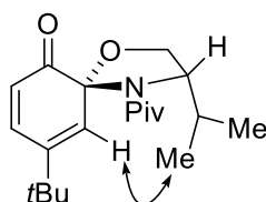
Figure 1. NOE correlation observed in the NOESY spectra of 29
