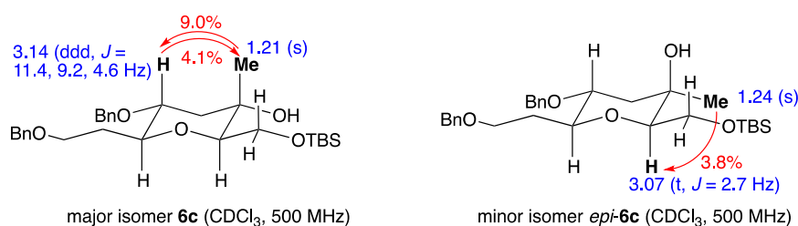
Figure 2. Difference NOE experiments for 6c and epi-6c
