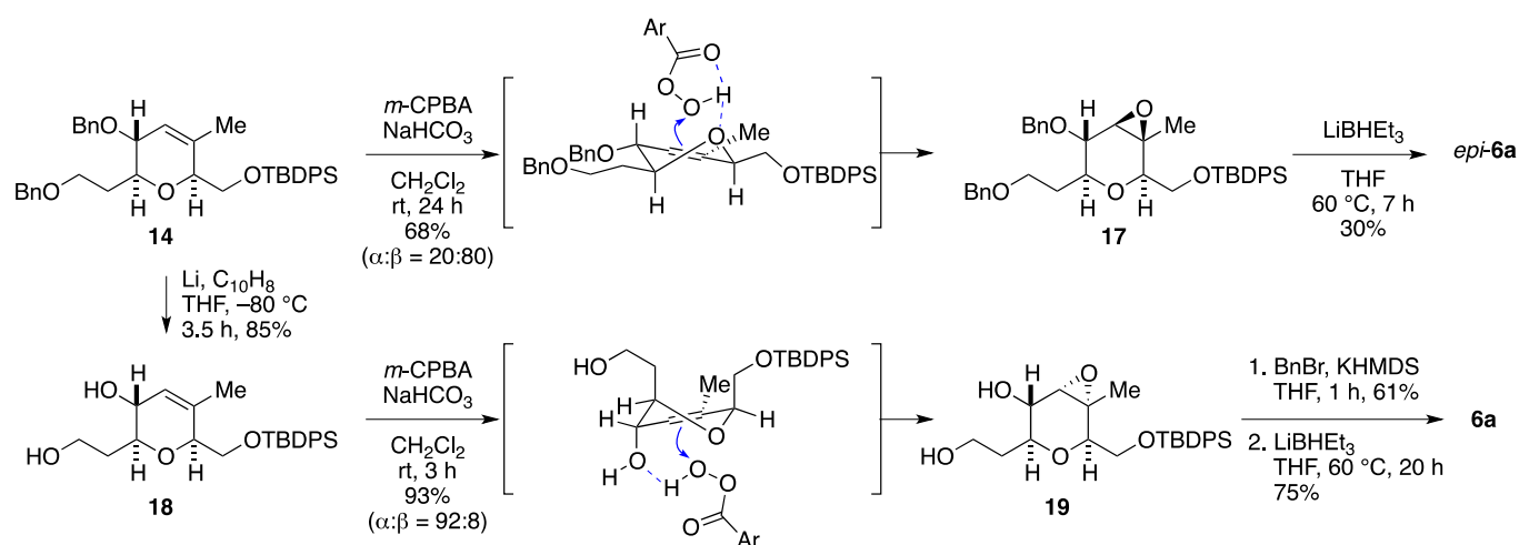
Scheme 5. Conversion of olefin 14 to 6a through neighboring group-assisted epoxidation followed by superhydride reduction
