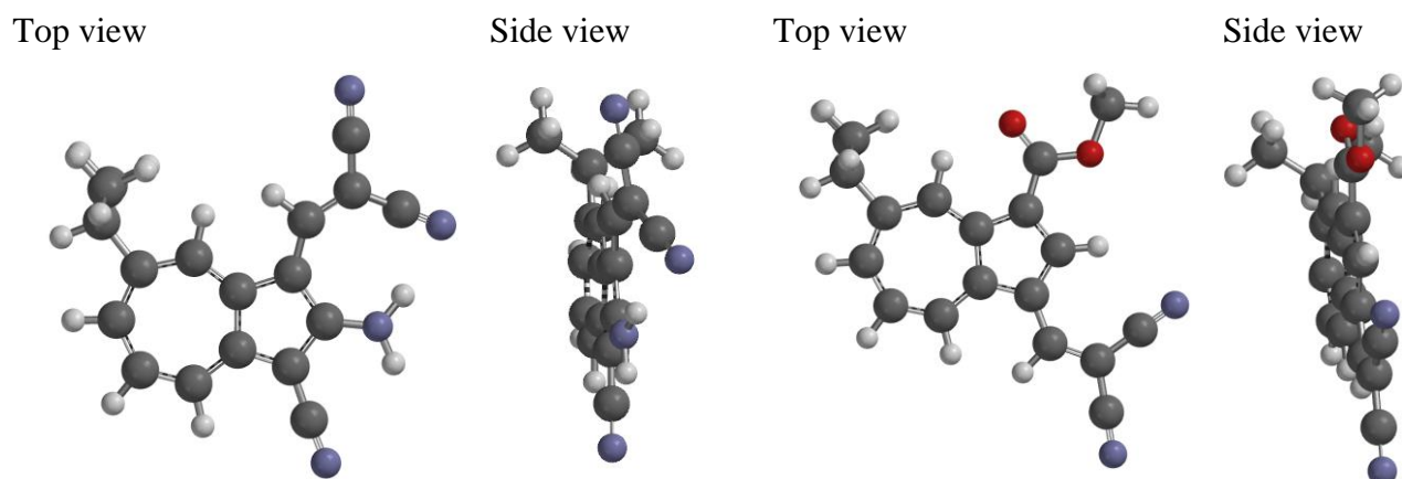
Figure 6. Optimized structure of 19 calculated by B3LYP/6-31G** level
