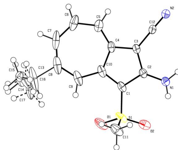
Figure 2. ORTEP drawing of 14b ; ellipsoids are drawn at the 50% probability level; Pbcn; a=9.9716(3)\text{ \AA} , b=16.6939(7)\text{ \AA} , c=16.7630(6)\text{ \AA} , \alpha=90^\circ , \beta=90^\circ , \gamma=90^\circ ; V=2790.45(18)\text{ \AA}^3 ; Z=8 ; D_{\text{calcd}}=1.373\text{ g cm}^{-3} ; \mu(\text{Mo-K}\alpha)=2.346\text{ cm}^{-1} ; R_1 [I>2\sigma(I)]=0.0668 , wR_2 [\text{all data}]=0.1499
