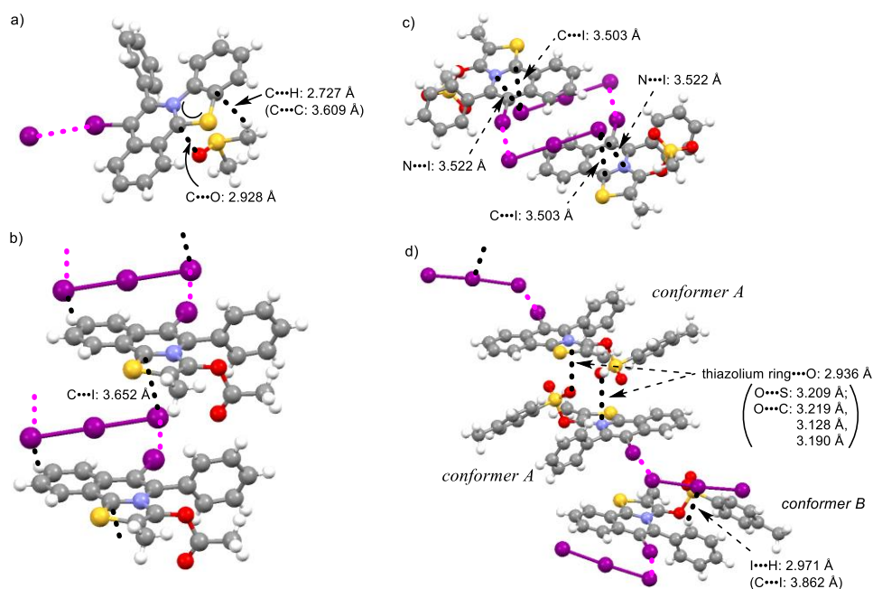
Figure 2. Electrostatic interaction in a) 2a^+ \cdot I^- \cdot DMSO , b) 2d^+ \cdot I_3^- , c) 2f^+ \cdot I_3^- , and d) 2g^+ \cdot I_3^- with selected distances. Purple dotted line represented I \cdots I interaction.
