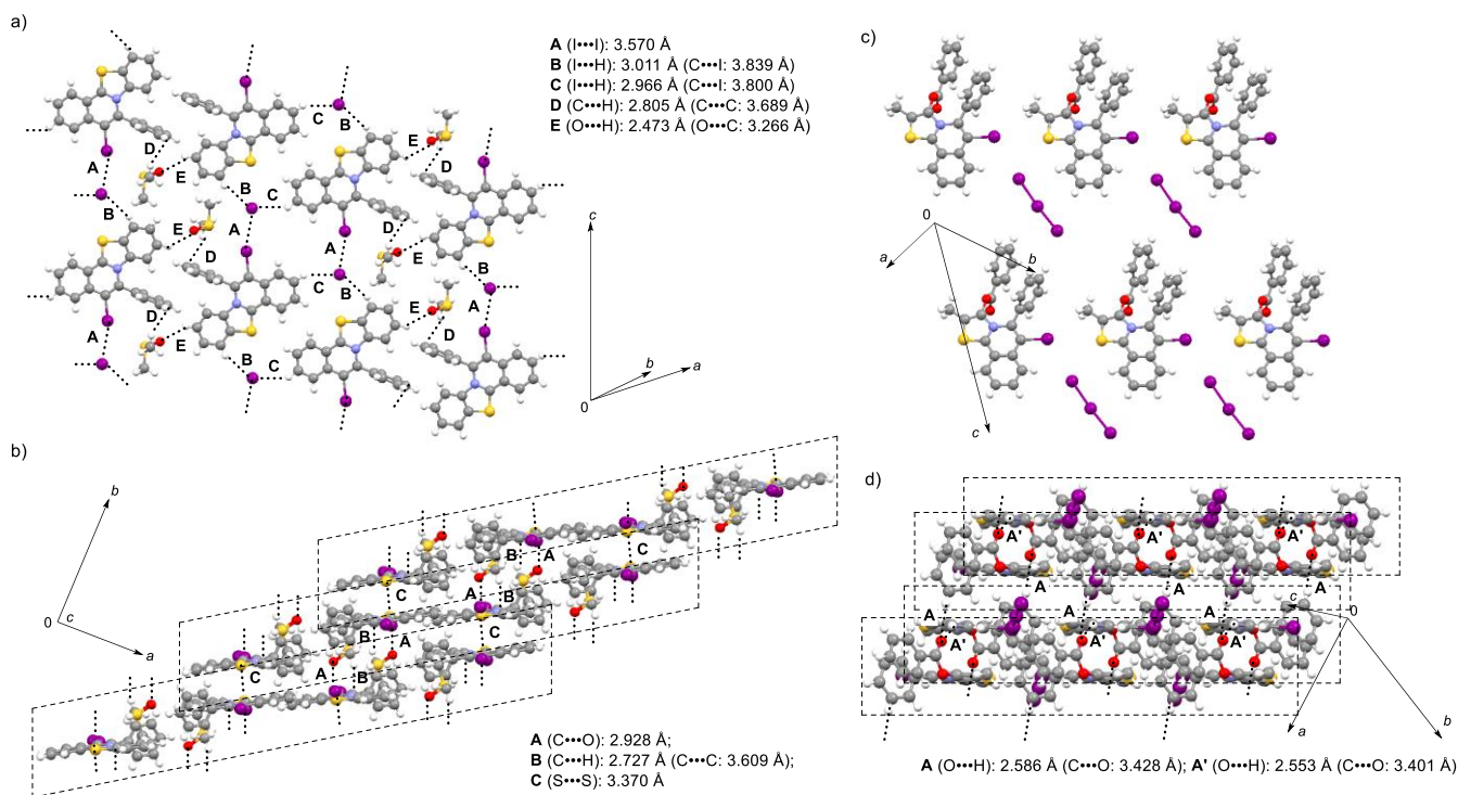
Figure 3. Sheet structures of a) 2\mathbf{a}^+\cdot\Gamma^- \cdot \text{DMSO} and c) 2\mathbf{e}^+\cdot\text{I}_3^- and the interactions between the layers of b) 2\mathbf{a}^+\cdot\Gamma^- \cdot \text{DMSO} and d) 2\mathbf{e}^+\cdot\text{I}_3^- with selected distances. One sheet was shown with frame in b) and d).
