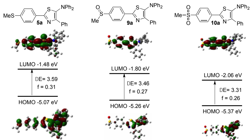
Figure 1. Energy levels and Kohn-Sham plots of HOMO and LUMO of 5a , 9a and 10a a a DFT, TD-DFT (TD/B3LYP/6-31+G(d,p)) calculations were carried out with the use of optimized structures at B3LYP/6-31+G(d,p). Gas-phase energies are shown.
