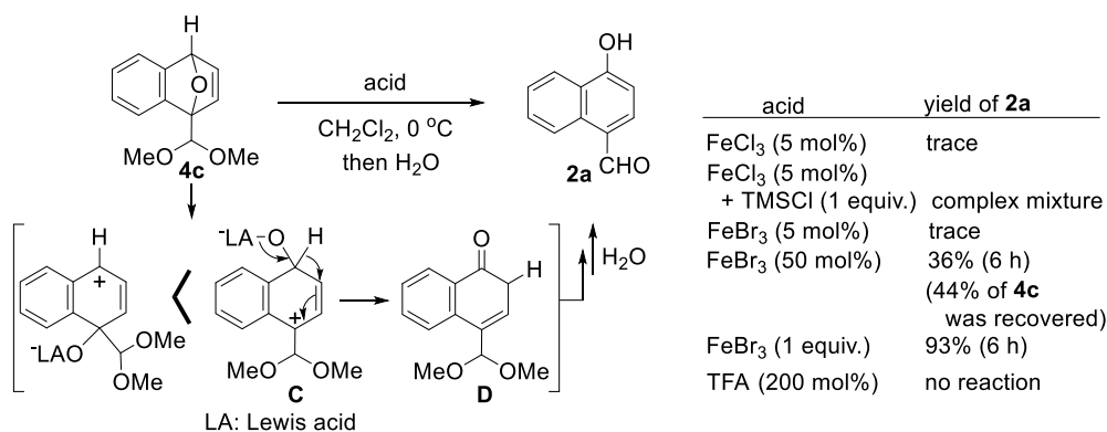
Scheme 3. Acid-catalyzed ring opening of 1-dimethoxymethyl-substituted 1,4-epoxy-1,4-dihydronaphthalene
