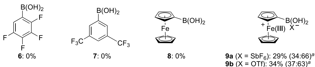
(b) Screening of bifunctional arylboronic acids
