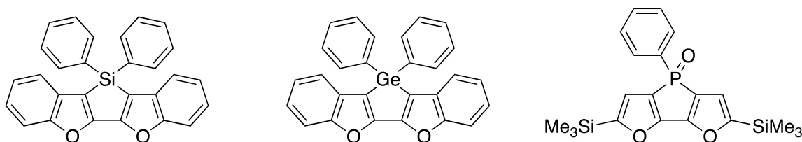
Figure 1. Furan-fused heteroaromatic compounds
