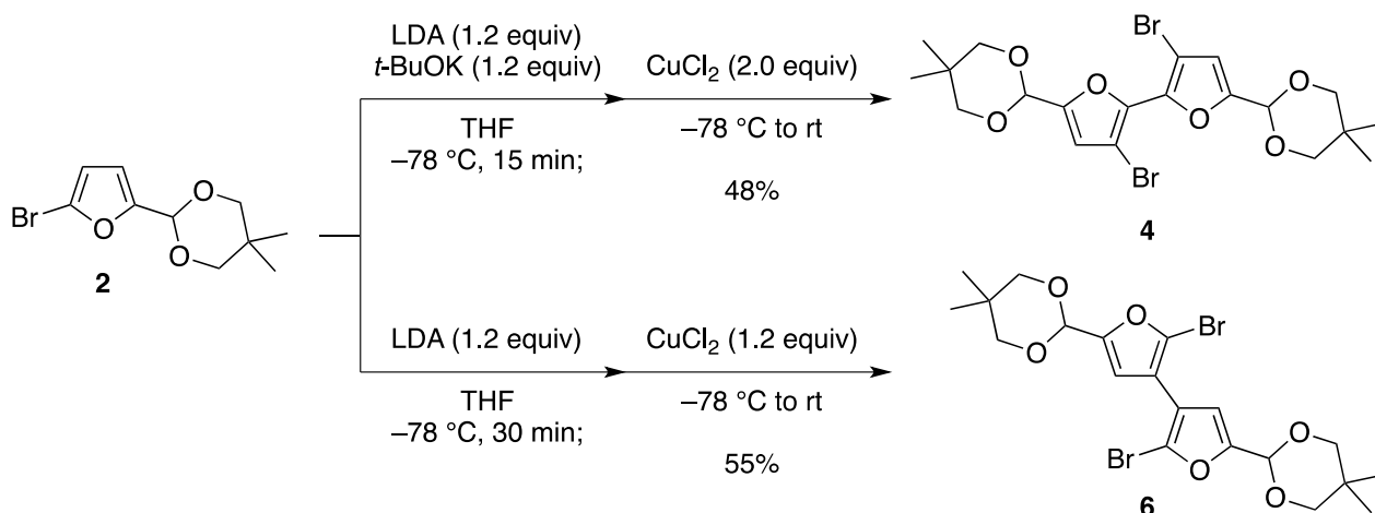
Scheme 2. Oxidative formation of furan dimers
