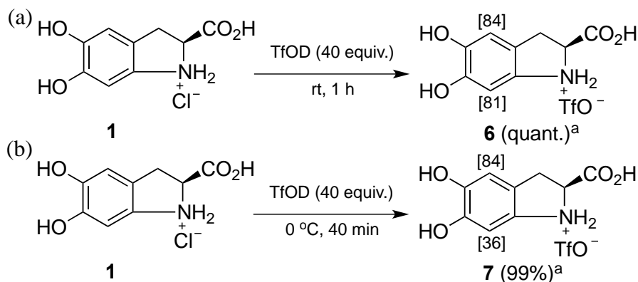
Scheme 4. Synthesis of deuterated cDOPA derivatives ( 6 and 7 )
