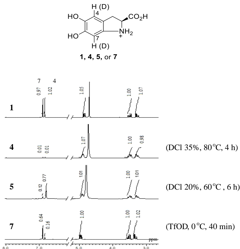
Figure 4. Selected ^1\text{H-NMR} profile of cDOPA ( 1 ) and deuterated cDOPA derivatives ( 4–5, 7 )
