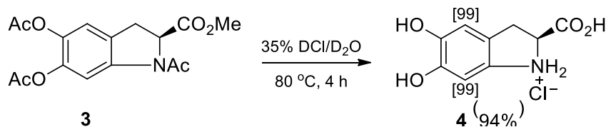
Scheme 2. Synthesis of deuterated cDOPA derivative ( 4 )
