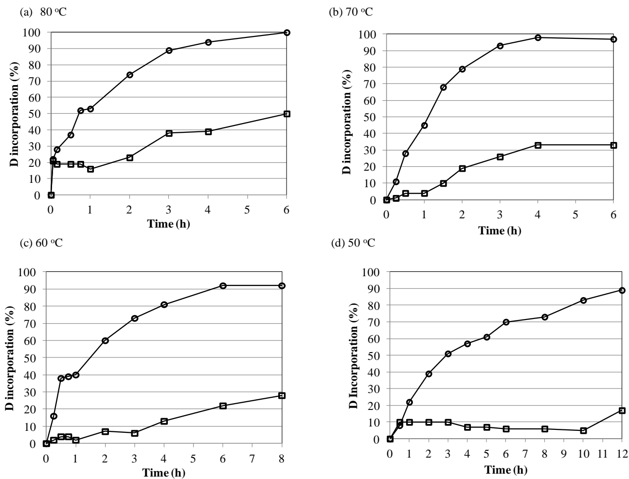
Figure 2. Hydrogen/deuterium exchange of cycloDOPA ( 1 ) by 20% DCl/D 2 O dependent on temperature of (a) 80 °C, (b) 70 °C, (c) 60 °C, and (d) 50 °C. The time-course H/D exchange was determined which –□– present for 4-position and –○– present for 7-position.
