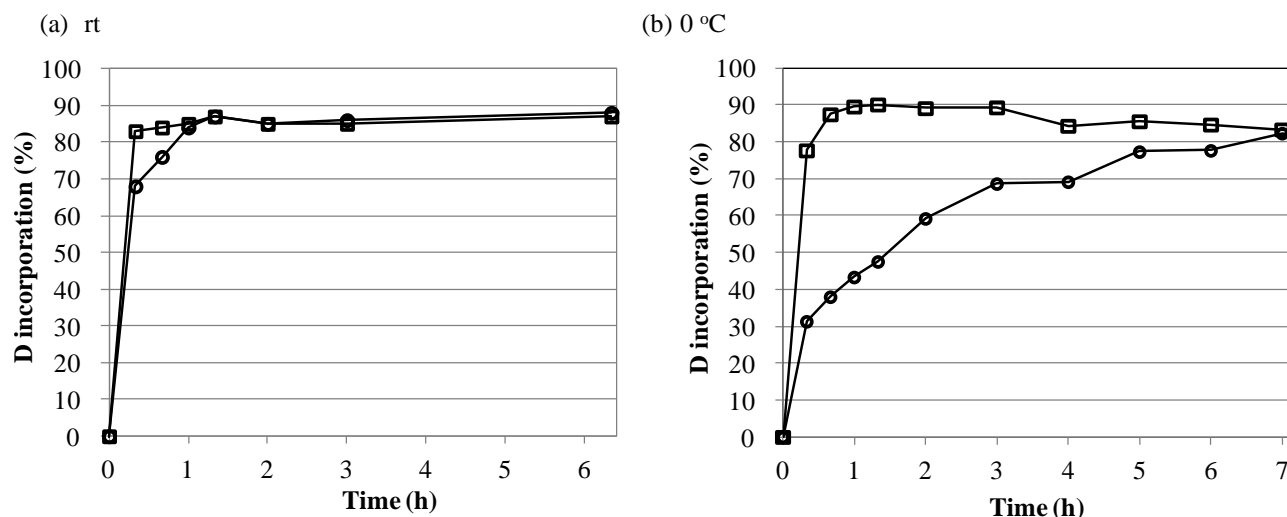
Figure 3. Hydrogen/deuterium exchange of cycloDOPA ( 1 ) with triflic acid (TfOD, 40 equiv.) at (a) rt and (b) 0 °C. The time-course H/D exchange was determined which \square — present for 4-position and \circ — present for 7-position.
