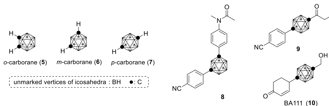
Figure 2. Structures of the three isomers of carborane and our developed carborane-based PR and AR antagonists
