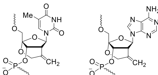
Figure 1. Structures of methylene-EoDNA-T and methylene-EoDNA-A
