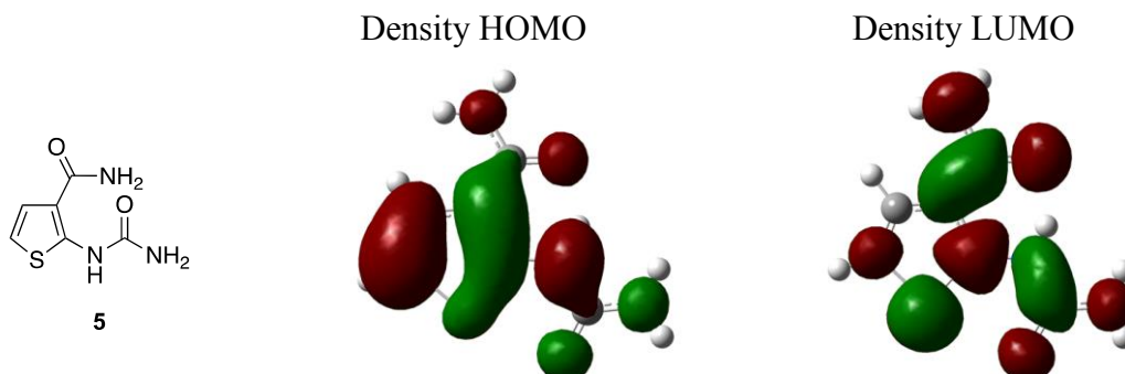
Figure 1. HOMO and LUMO densities of 5
