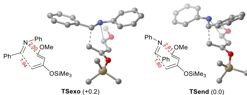
Figure 4. Three-dimensional (3D) structures and relative energies of TSexo and TSend in aza-Diels-Alder reaction (B3LYP/6-31+G**)
