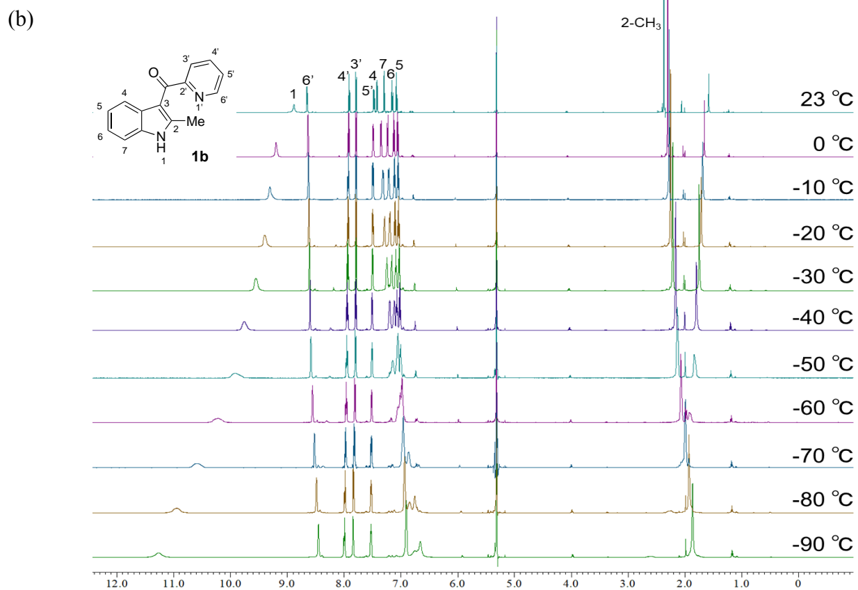
Figure 5. VT-NMR of 1b (a): +23 °C ~ +120 °C in DMSO- d 6 ; (b): -90 °C ~ +23 °C in CD 2 Cl 2
