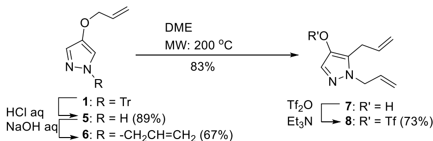
Scheme 2. Synthesis of RCM substrates 7 and 8 from 4-allyloxy-1H-1-tritylpyrazole ( 1 )
