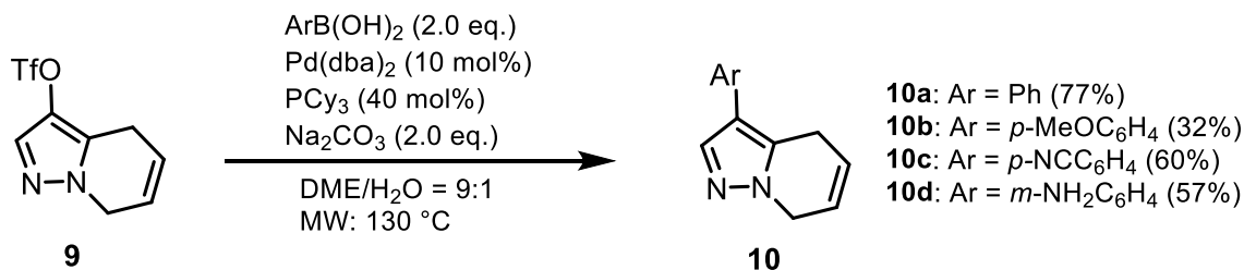
Scheme 4. Suzuki-Miyaura coupling of triflate 9 and arylboronic acids using the reported conditions
