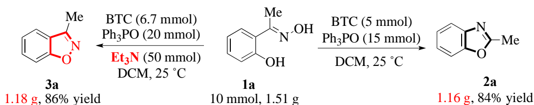
Scheme 1. Higher-Scale Reaction
