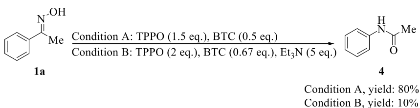
Scheme 2. Control experiments
