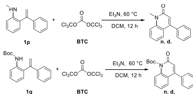
Scheme 3. Control experiments
