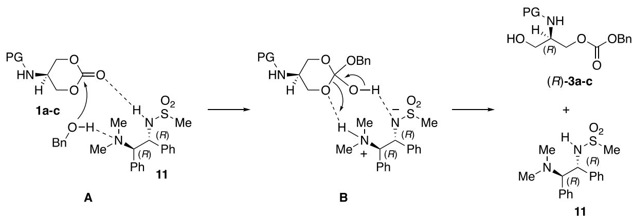
Figure 1. A plausible activation mode for the catalytic asymmetric ring-opening of \sigma -symmetric cyclic carbonates 1a–c with chiral amino sulfonamide catalyst 11
