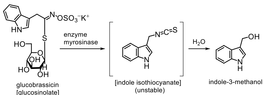
Scheme 1. Reaction of glucobrassicin catalyzed by enzyme myrosinase
