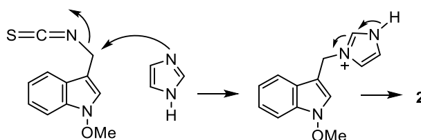
Scheme 4. Plausible reaction mechanism for the synthesis of 2
