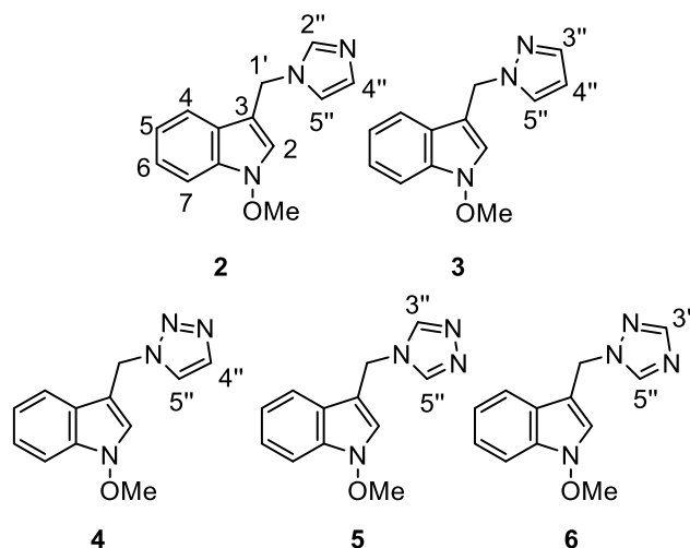
Scheme 3. Structure of compounds 2-6
