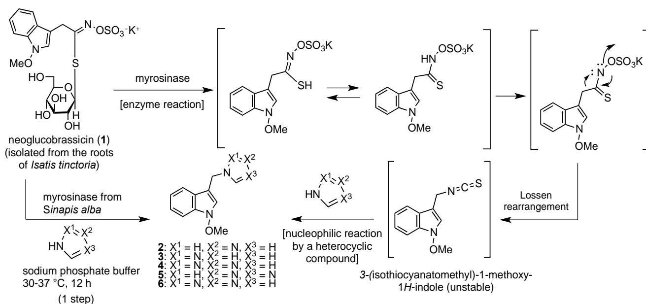
Scheme 2. Construction of 1-methoxyindoles with a heterocyclic moiety
