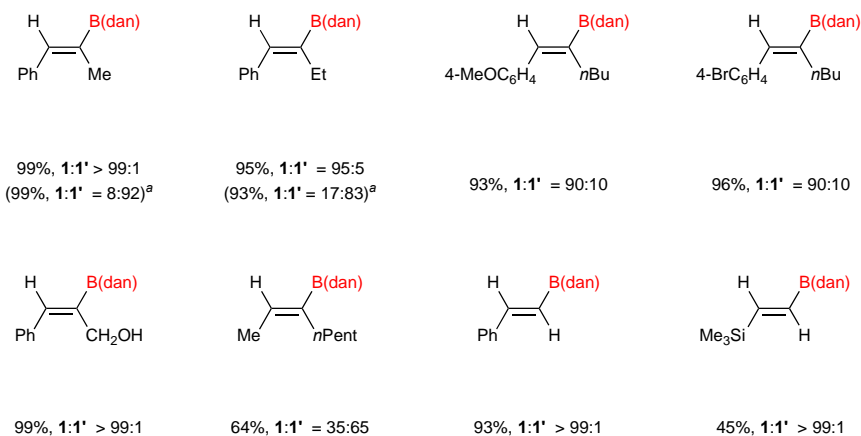
Scheme 9
