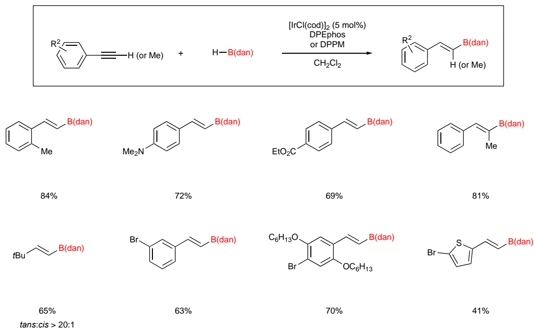
Scheme 50
