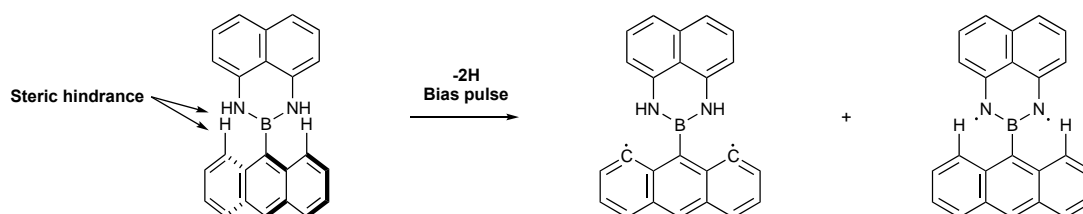
Scheme 27
