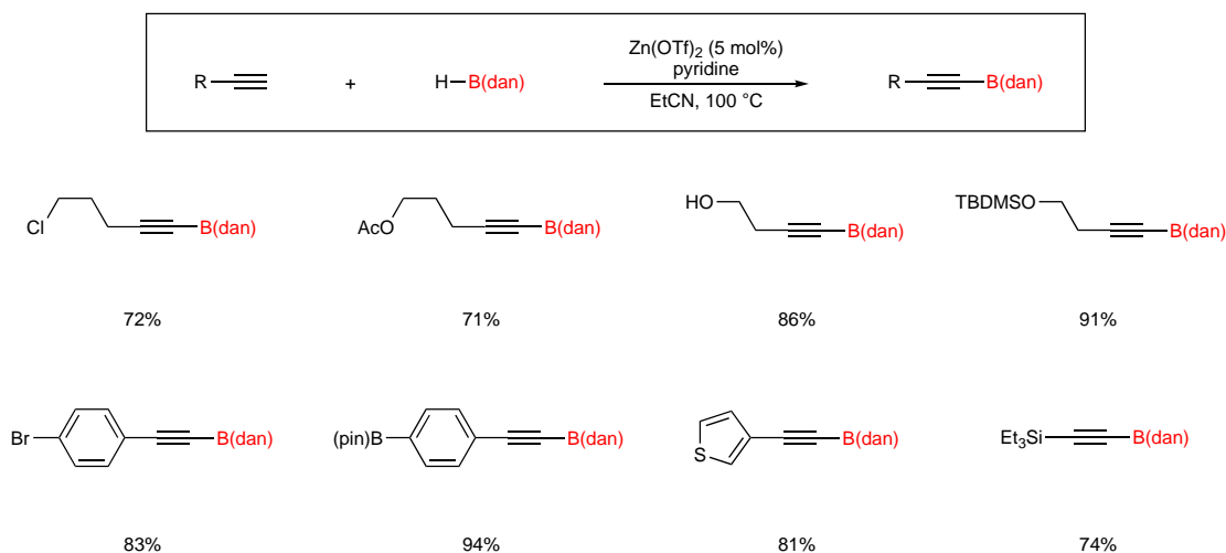
Scheme 57
