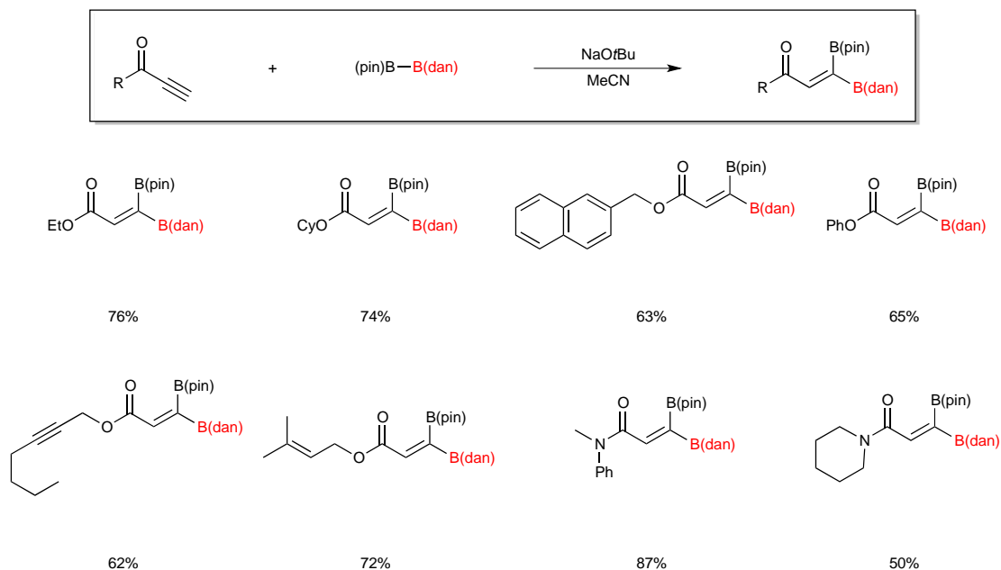
Scheme 46
