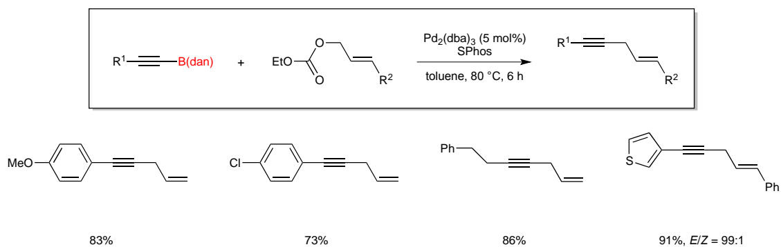
Scheme 65
