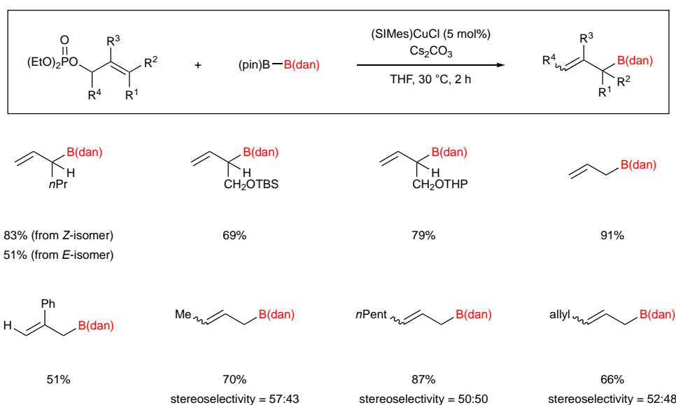
Scheme 31
