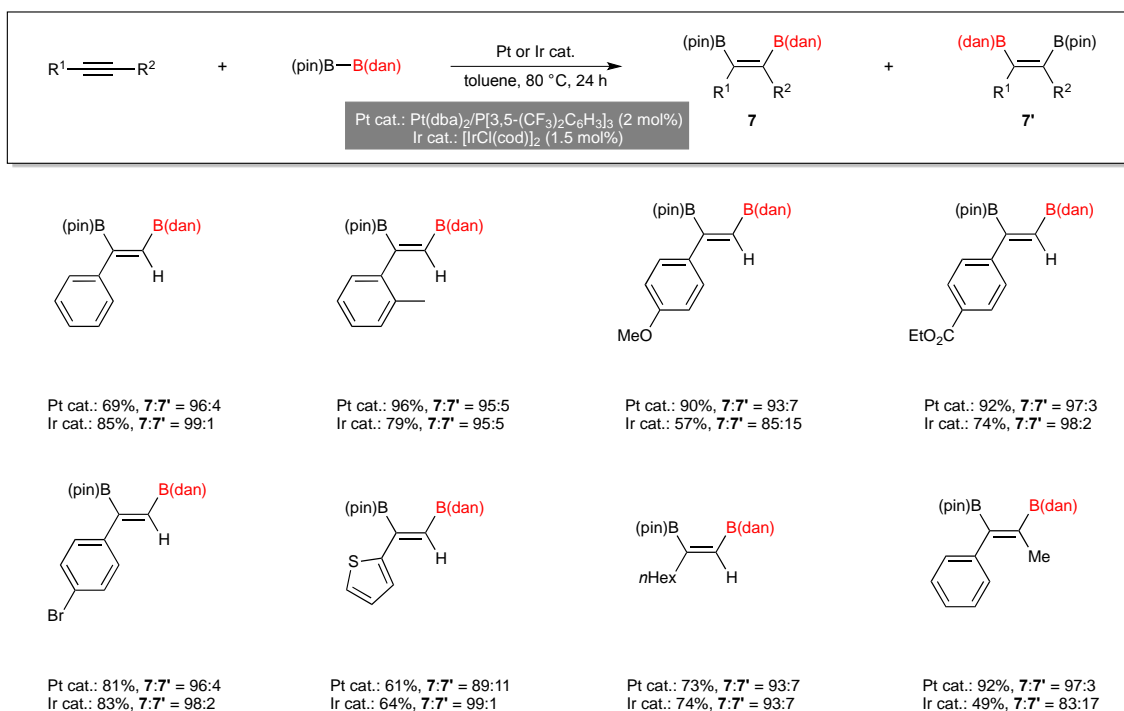
Scheme 38
