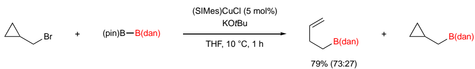
Scheme 29
