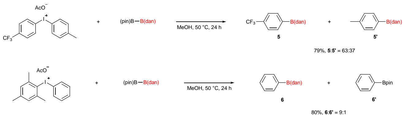
Scheme 36
