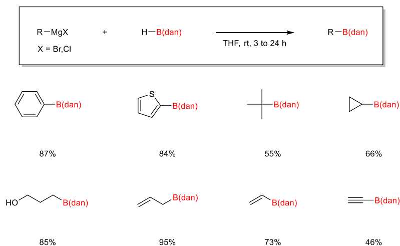
Scheme 59
