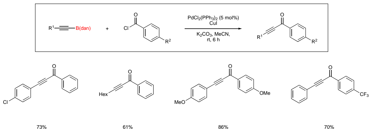
Scheme 66
