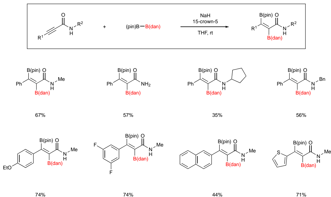
Scheme 42
