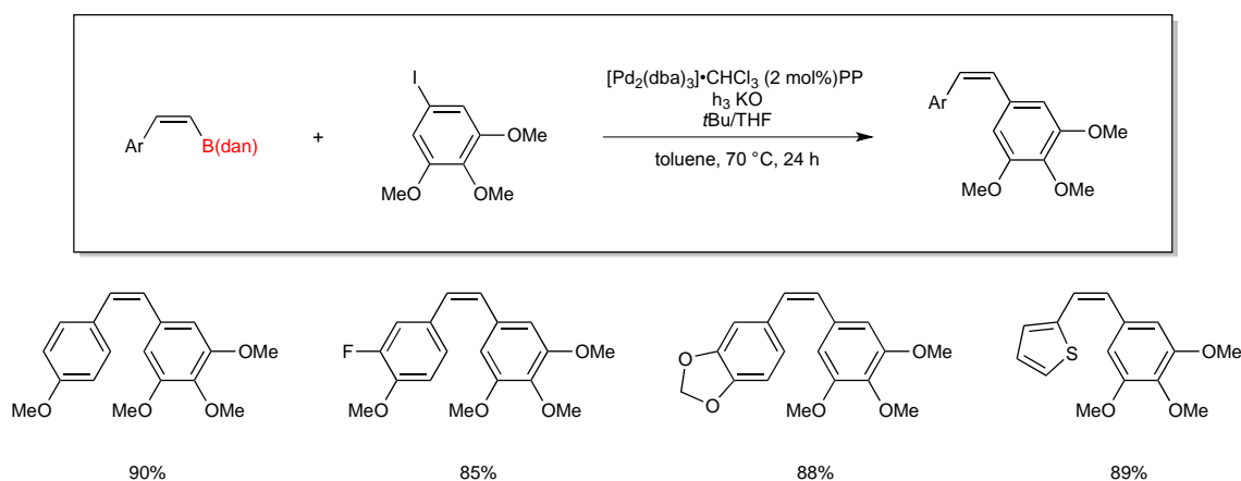
Scheme 67
