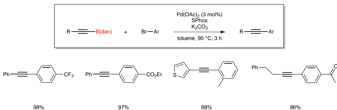
Scheme 64
