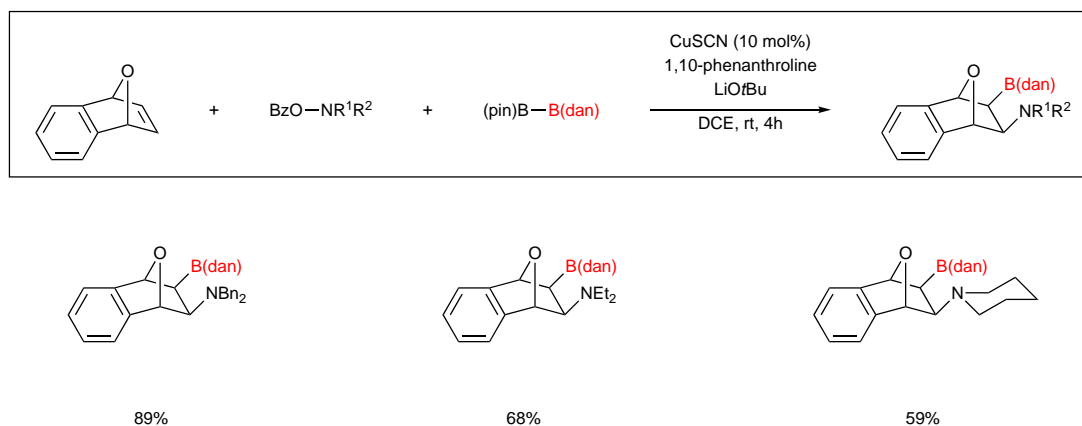
Scheme 21
