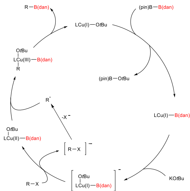
Scheme 30
