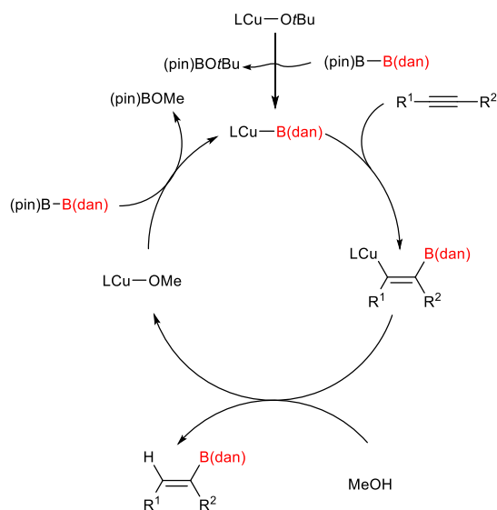
Scheme 10
