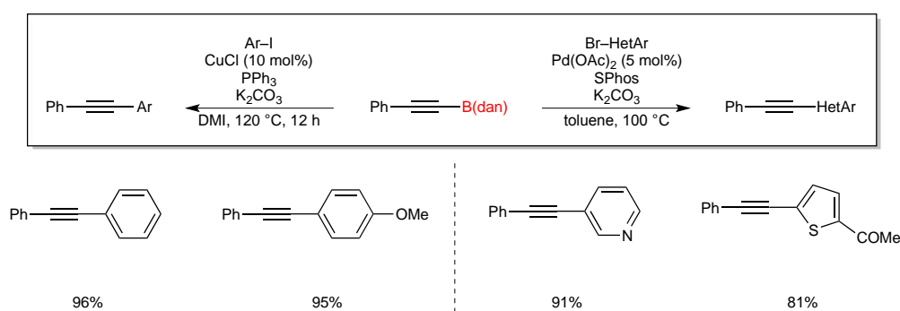
Scheme 63
