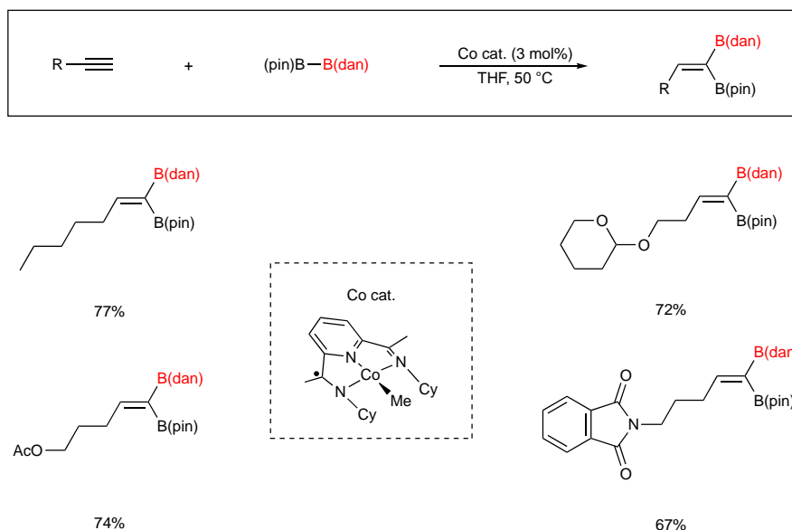
Scheme 48
