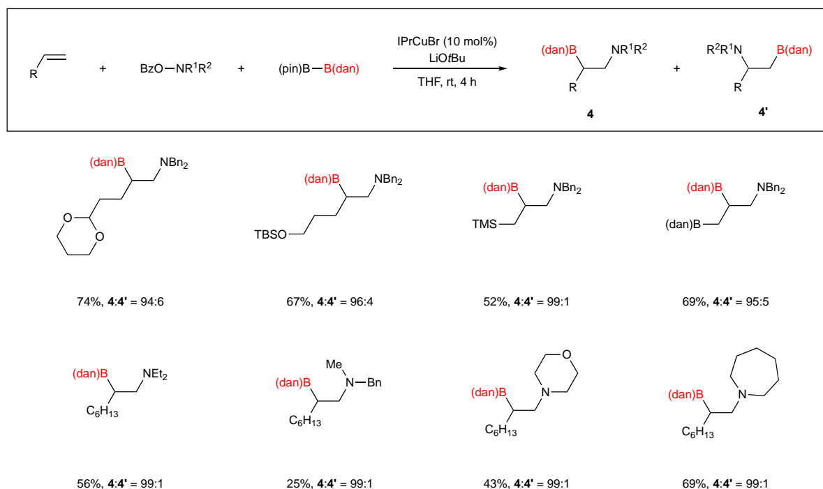
Scheme 22
