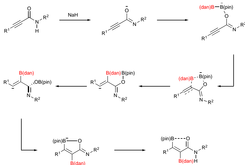
Scheme 43
