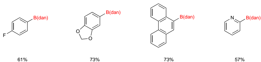
Scheme 28
