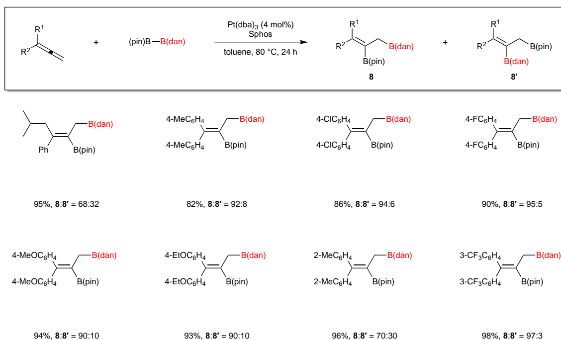
Scheme 39
