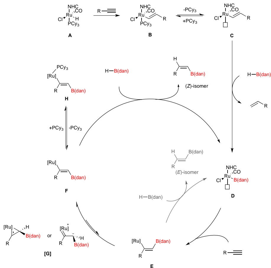
Scheme 54
