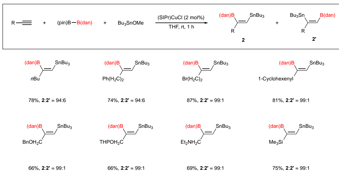
Scheme 16
