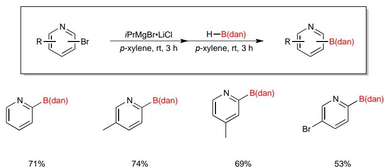
Scheme 60
