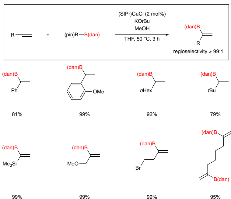
Scheme 8
