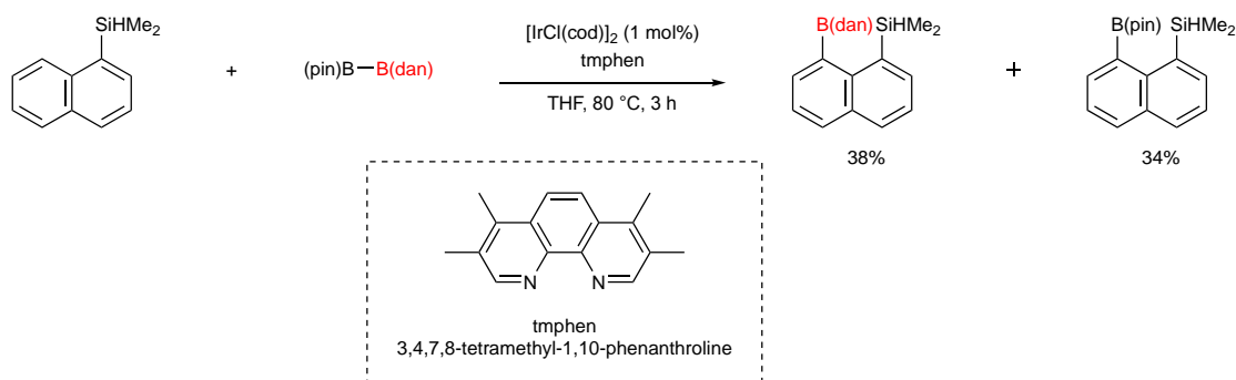
Scheme 37
