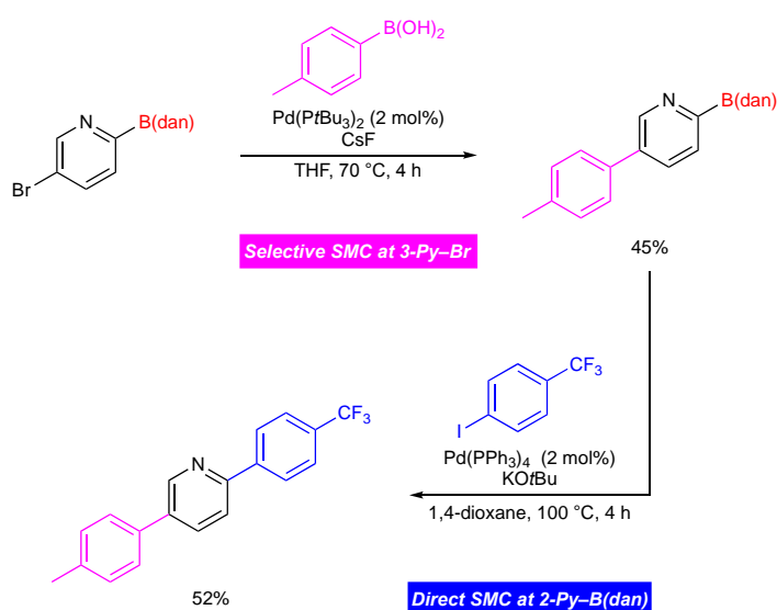
Scheme 71
