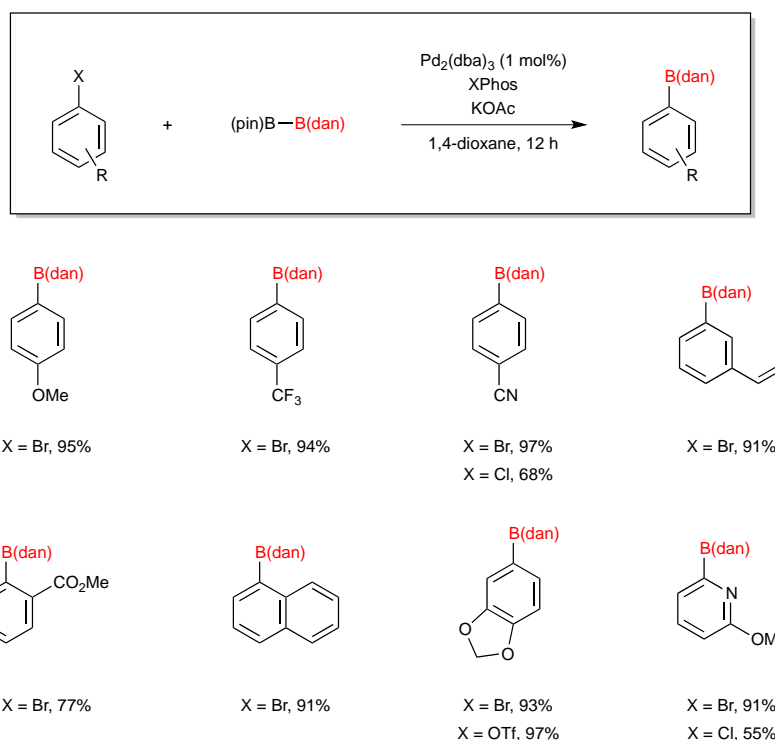
Scheme 23
