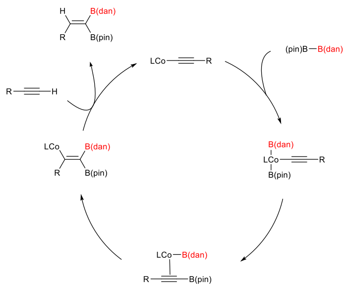
Scheme 49
