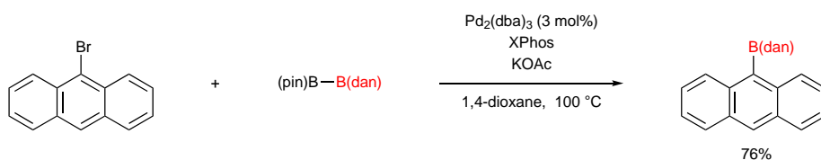
Scheme 26
