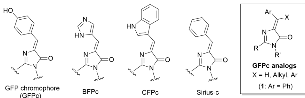
Figure 1. Structures of green fluorescent protein chromophore (GFPc) and its analogs
