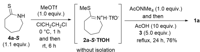
Scheme 2. Synthesis of 1a from thiolactam 4a-S
