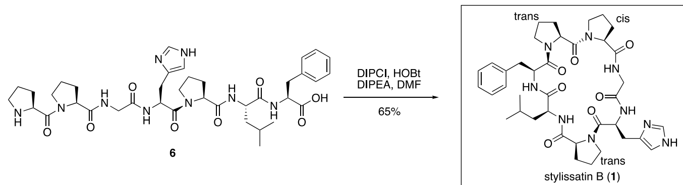
Scheme 2. Synthesis of stylissatin B ( 1 )
