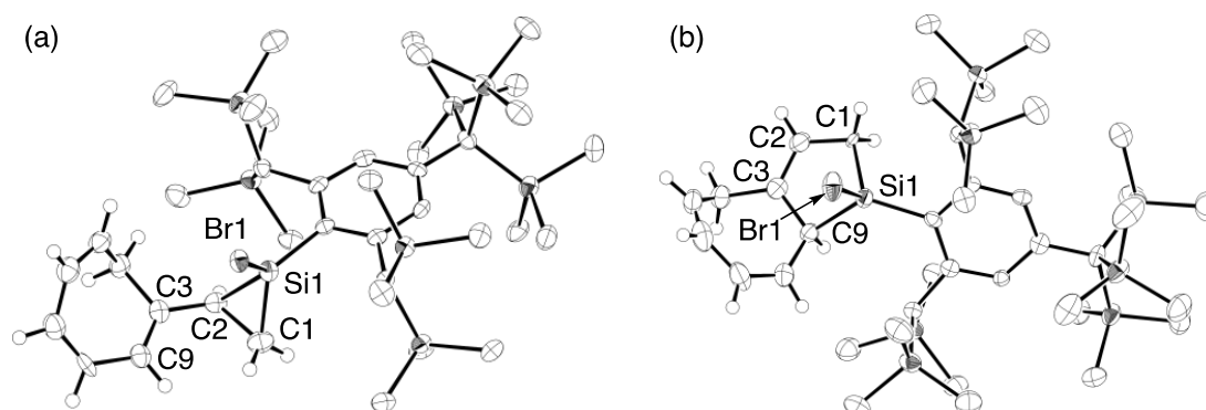
Figure 1. Thermal ellipsoid plots (50% probability) of compounds 5 (a) and 6 (b). Hydrogen atoms on Bbt substituents were omitted for clarity.
