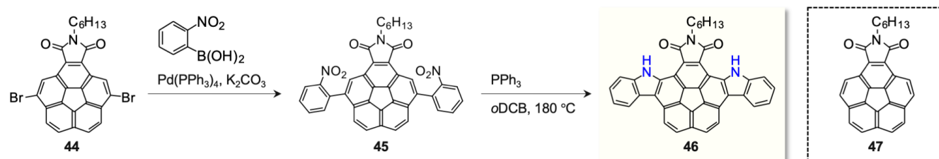
Scheme 6. Indole fused corannulene imide
