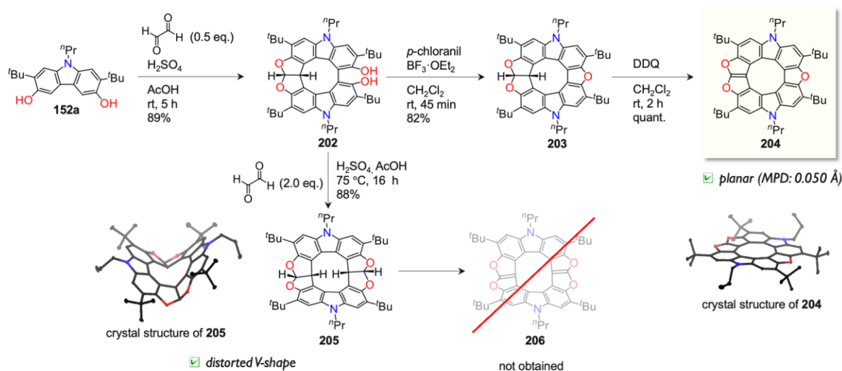
Scheme 24. Synthesis of diazatrioxa[9]circulene and attempted synthesis of [10]circulene
