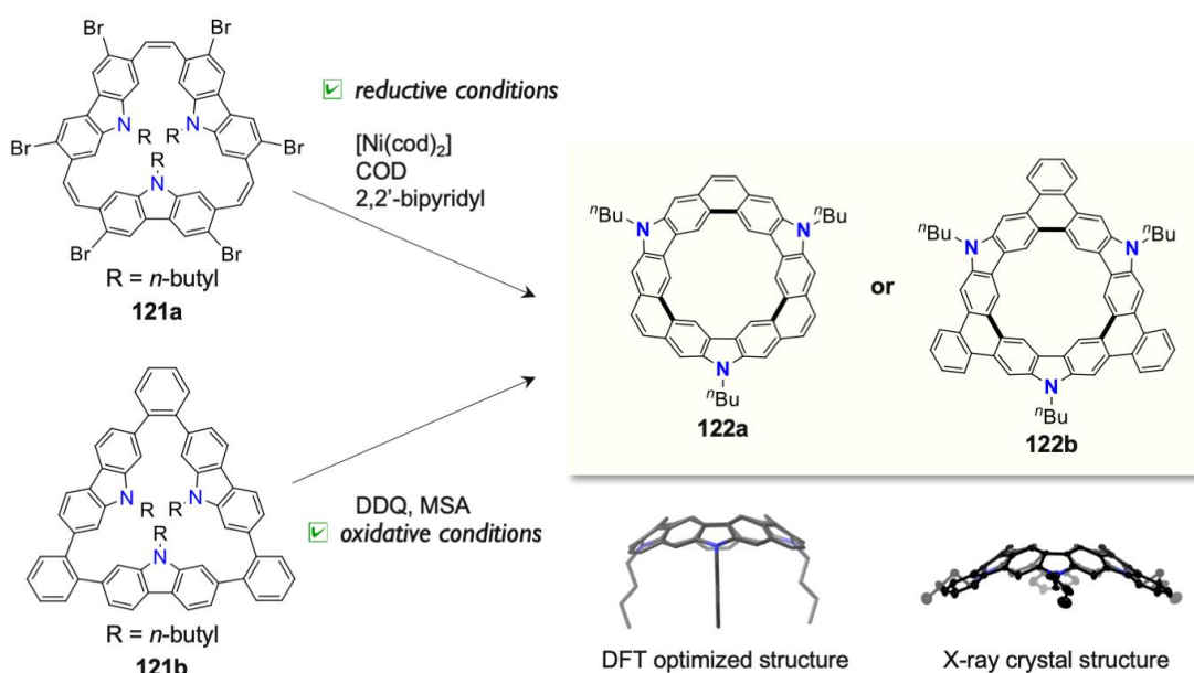
Scheme 14. “Fold-in” type synthesis toward bowl shaped cyclic PAHs
