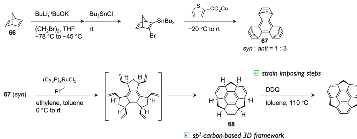
Scheme 9. The synthesis of sumanene
