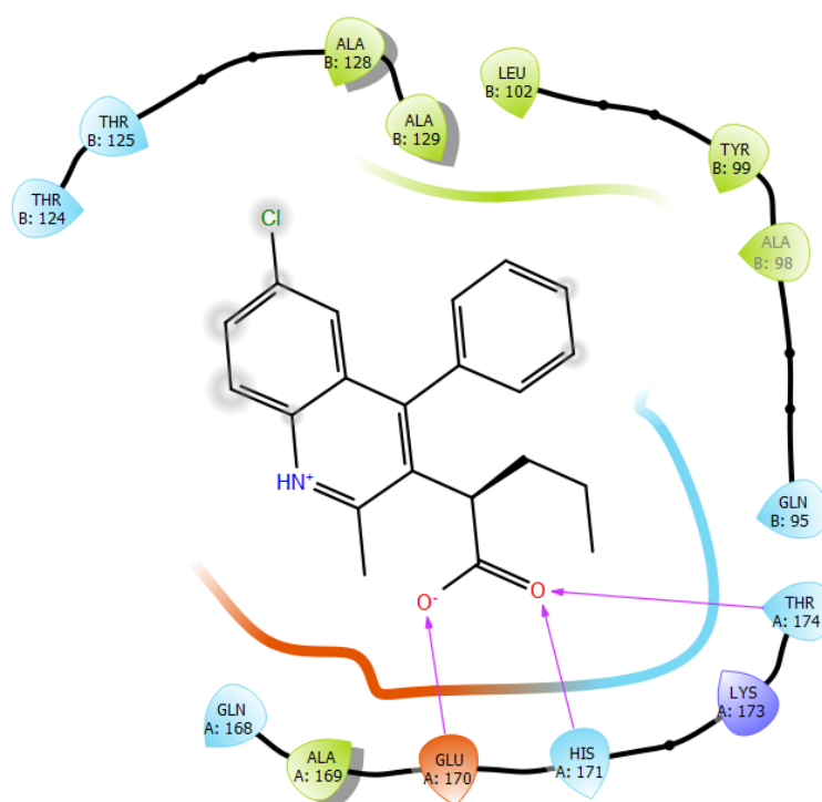
Figure 3. 2D binding mode of CX05168 in the LEDGF/p75 binding site of HIV-1-IN
