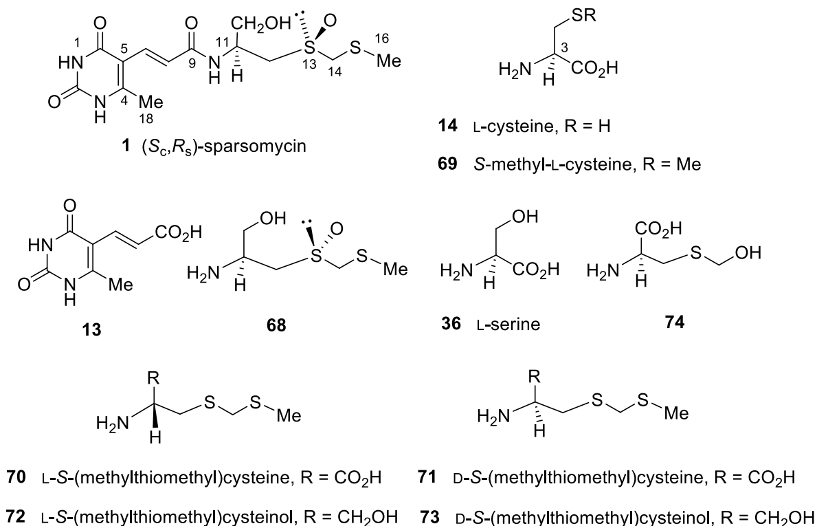
Figure 9. Potential precursors in the biosynthesis of sparsomycin ( 1 ) 83
