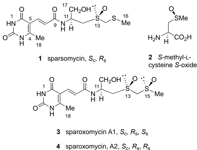
Figure 1. Structures of sparsomycin ( 1 ), S -methyl-L-cysteine- S -oxide ( 2 ), and the sparoxomycins A1 ( 3 ) and A2 ( 4 )
