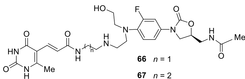
Figure 8. Linezolid analogs 66 and 67 of the uracil acrylic acid 13 47
